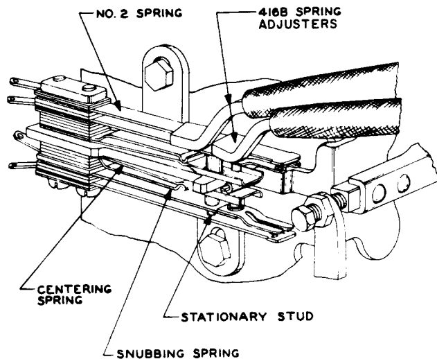
Fig. X—Method of Adjusting No. 2 Spring for Contact Separation and Front Contact Make
