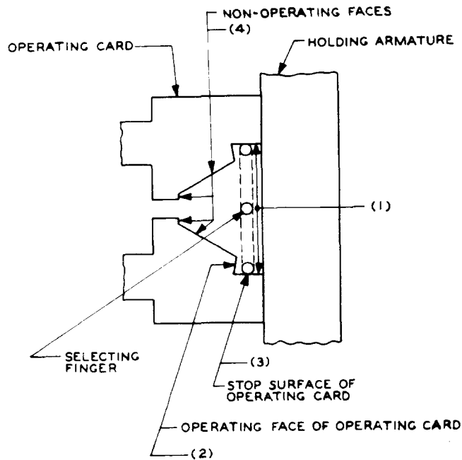
Fig. F—Position of Selecting Finger
