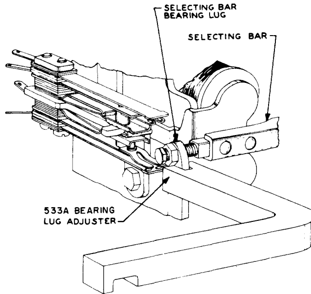
Fig. R—Method of Adjusting Selecting Bar Bearing Lug to Eliminate Bind
