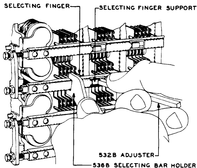
Fig. U—Method of Adjusting Selecting Finger Support
