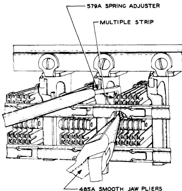
Fig. Y--Method of Adjusting Contact Multiple
