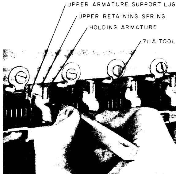
Fig. AA—Method of Adjusting Upper Armature Support Lug
