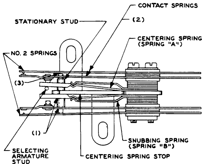
Fig. K—Selecting Off-Normal Spring Assembly With Selecting Unit Operated
