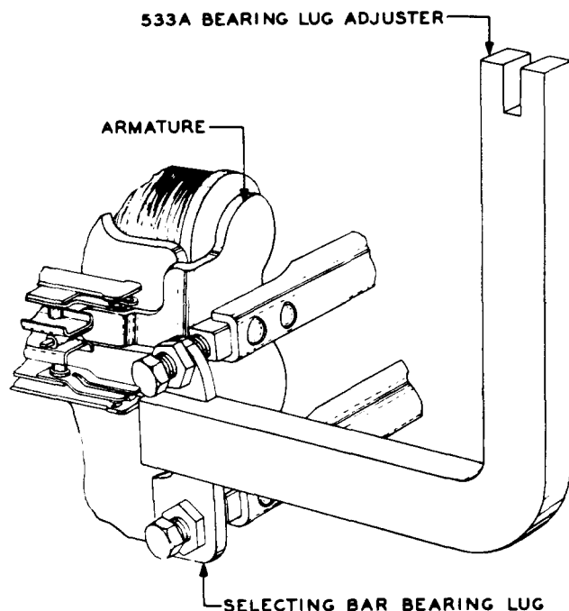
Fig. T—Method of Adjusting Selecting Bar Bearing Lug for Armature Travel
