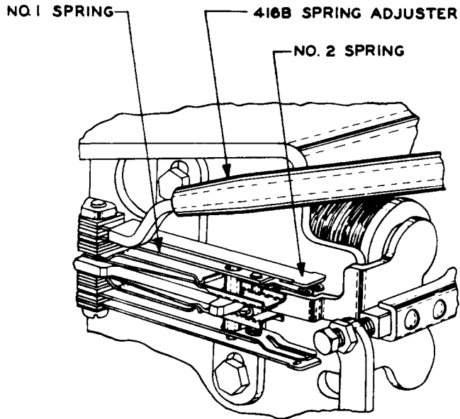
Fig. W—Method of Adjusting Springs for Straightness and Clearance
