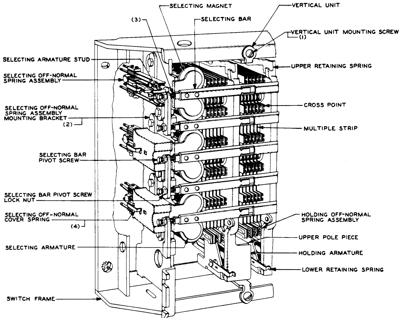
Fig. A—General View of Switch
