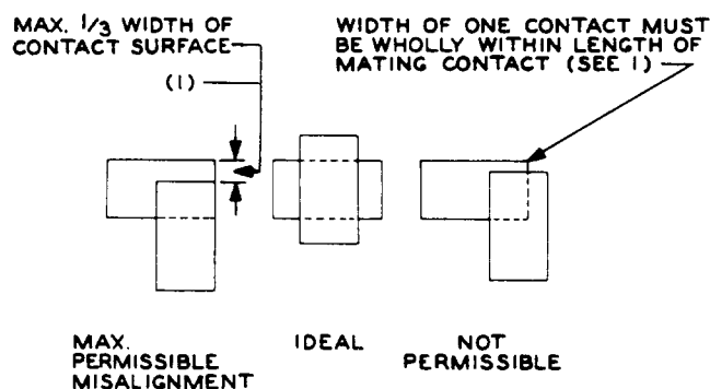
Fig. J—Alignment of Heavy Contacts—Plan View of Contact Surfaces
