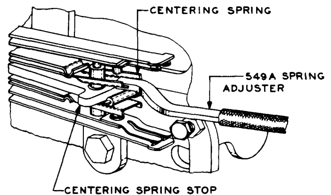
Fig. S—Method of Adjusting Centering Spring
