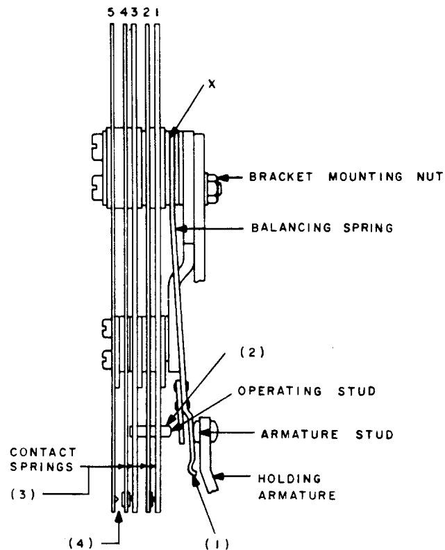
Fig. Q—Holding Off-Normal Spring Assembly
