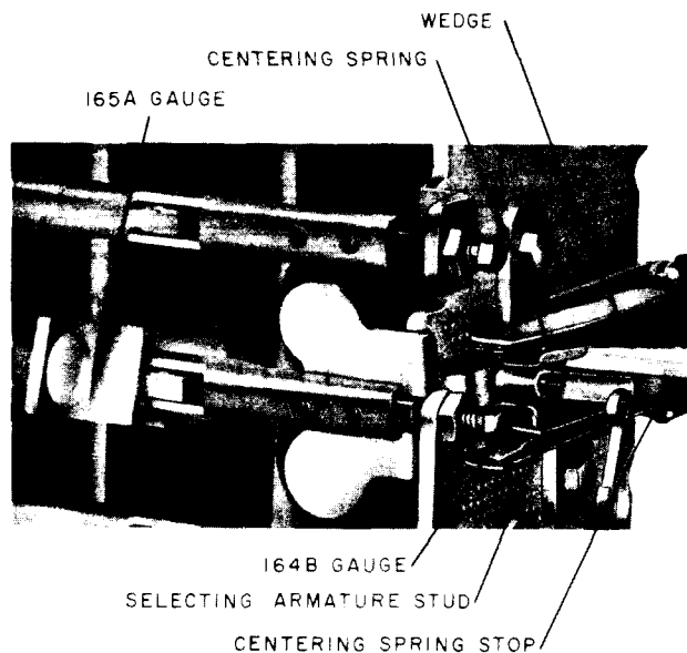
Fig. G—Method of Checking Position of Selecting Finger Using the 164B and 165A Gauges
