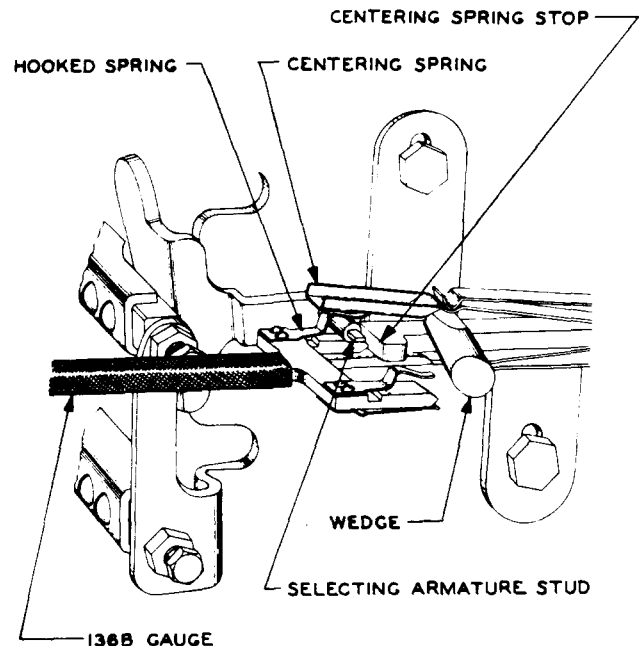
Fig. H—Method of Checking Position of Selecting Finger Using the 136B Gauge
