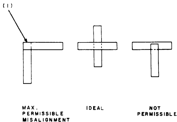
Fig. I—Alignment of Standard Contacts—Plan View of Contact Surfaces
