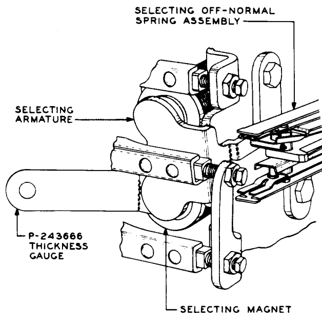
Fig. M—Method of Checking Front Contact Make on Selecting Off-Normal Spring Combination Fig. 104
