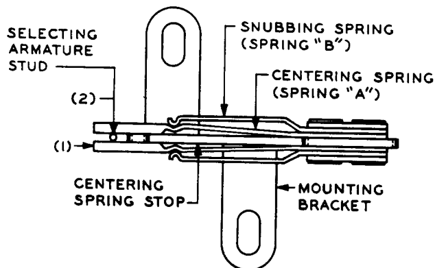
Fig. C—Centering Unit in Normal Position
