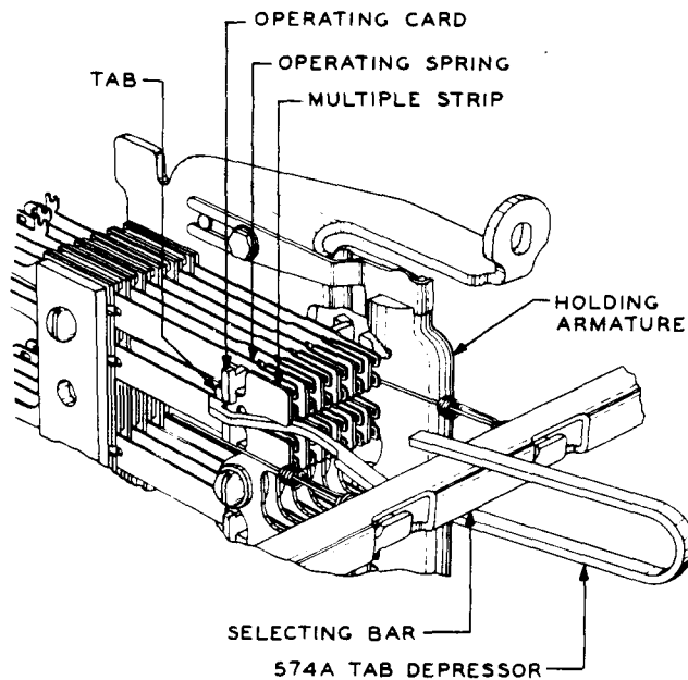
Fig. N—Method of Checking Operating Spring Pressure
