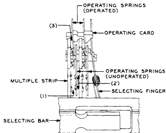
Fig. O—Clearance Between Operating Springs and Multiple Strip (Holding Armature Not Shown)
