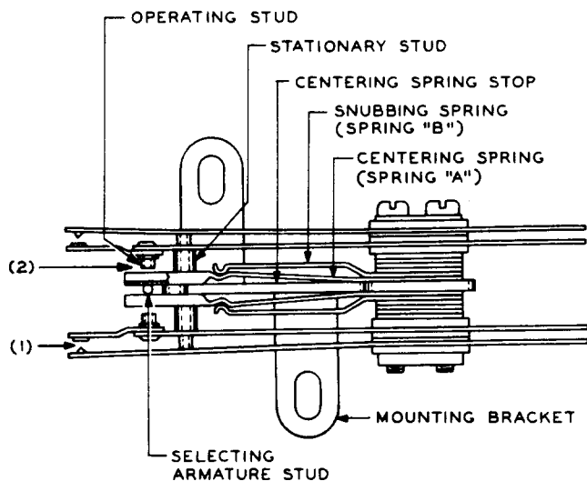
Fig. L—Selecting Off-Normal Spring Assembly With Selecting Unit Normal
