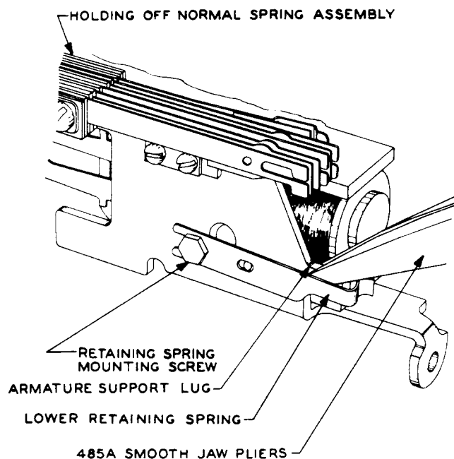
Fig. BB—Method of Adjusting Lower Armature Support Lug
