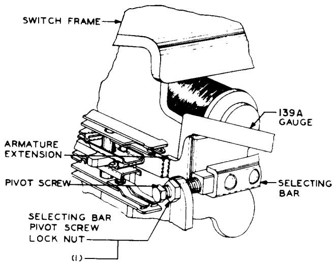
Fig. B—Method of Checking Clearance Between Wide Portion of Selecting Armature Extension and Switch Frame
