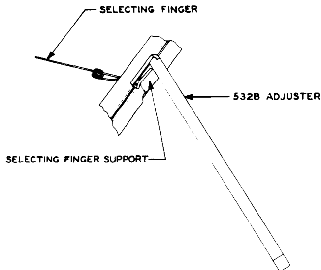
Fig. V—Method of Adjusting Selecting Finger to Left
