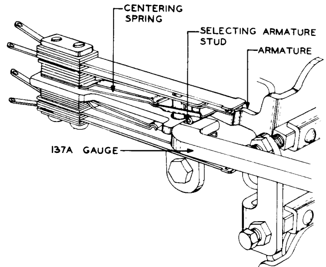
Fig. E—Method of Gauging Armature Travel
