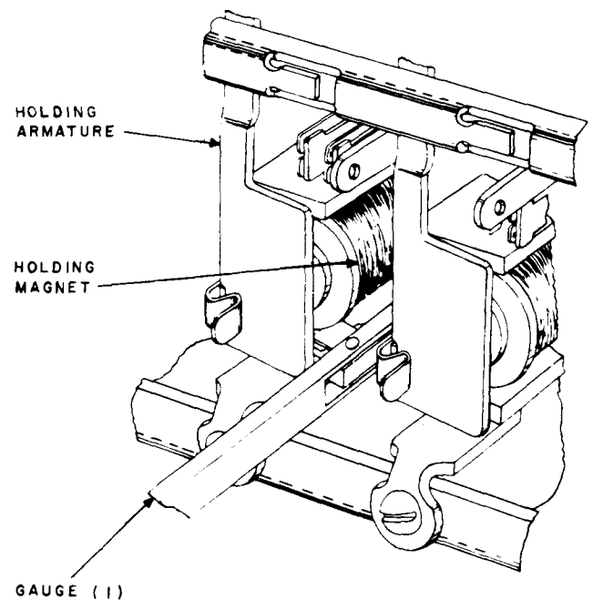
Fig. P—Method of Checking for Front Contact Make
