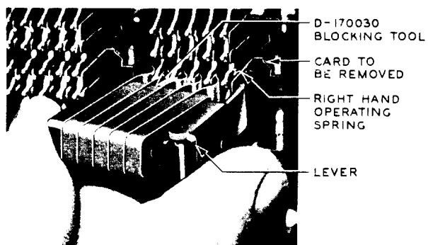
Fig. 5 - Applying Blocking Tool
