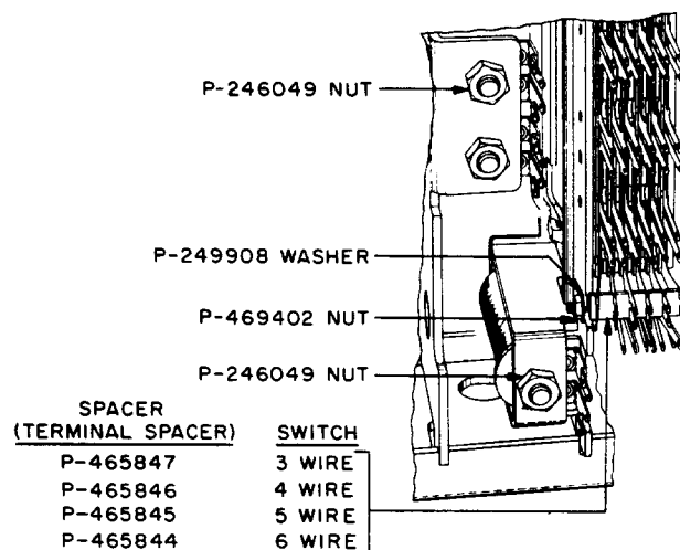
Fig. 2 - Partial Rear View of Switch Showing Magnet Mounting Part and Terminal Spacers
