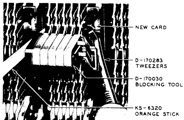
Fig. 10 - Final Positioning Operations of New Card
