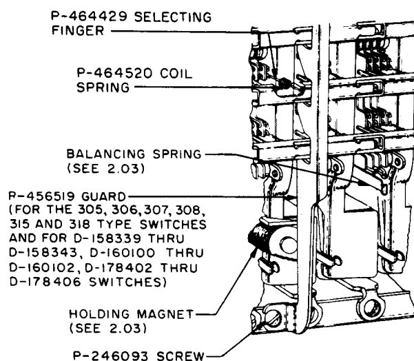
Fig. 3 - Partial Front View of Switch Showing Guard and Selecting Finger
