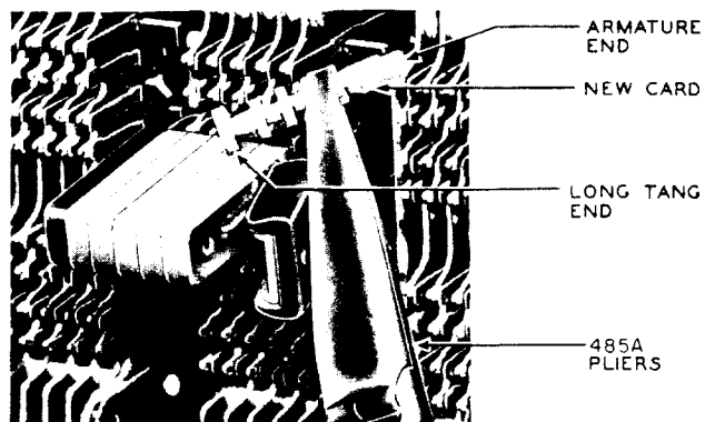
Fig. 8 - Grasping a New Card for Replacement
