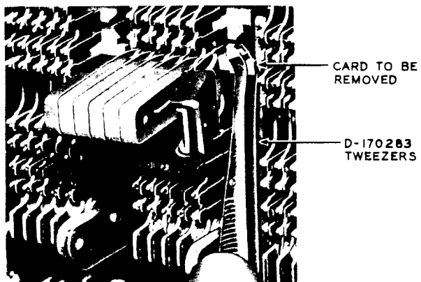
Fig. 7 - Rotating Card to a Flat Position With Tweezers
