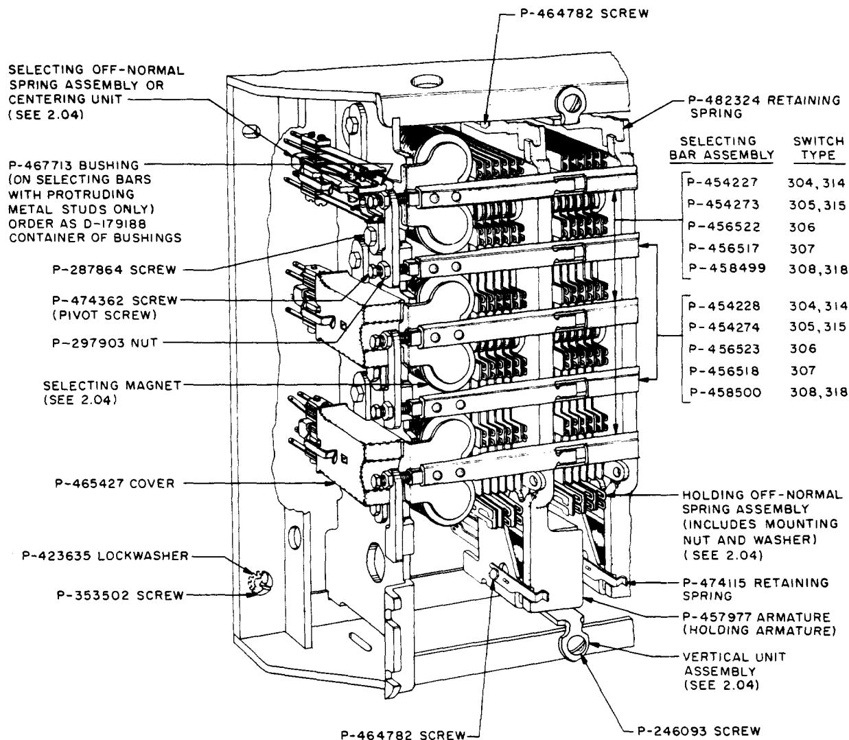
Fig. 1 - Front View of Switch
