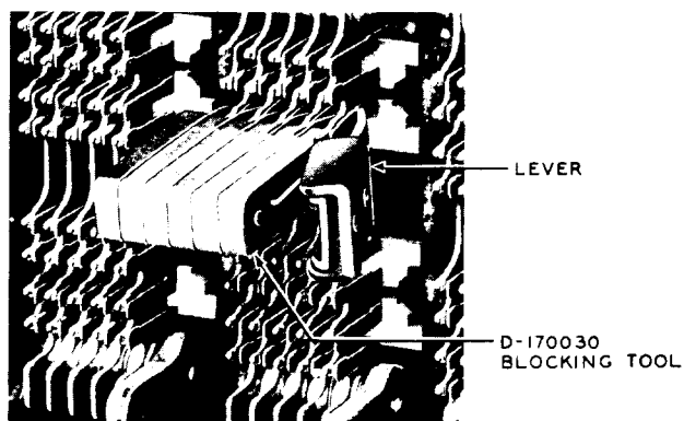
Fig. 6 - Blocking Tool in Position
