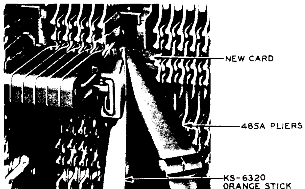
Fig. 9 - Inserting New Card in Spring Combination
