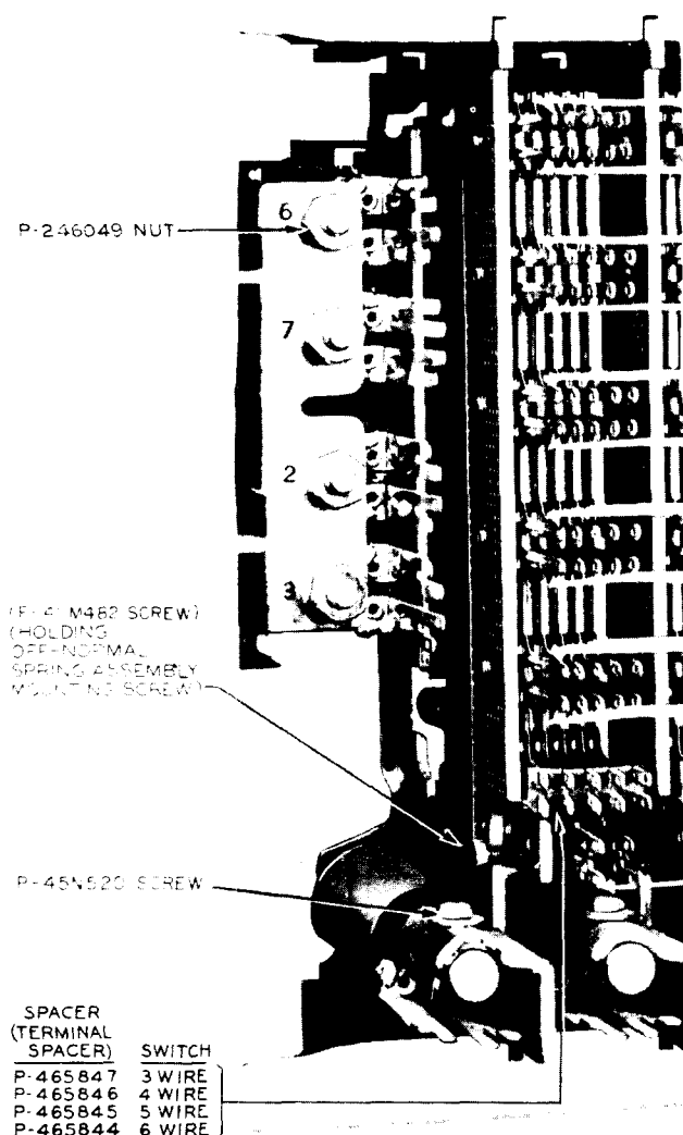
Fig. 2—Partial Rear View of Switch Showing Magnet Mounting Parts and Terminal Spacers
