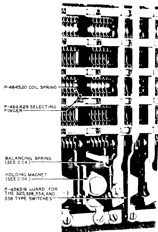
Fig. 3—Partial Front View of Switch Showing Vertical Unit With Holding Armature Removed
