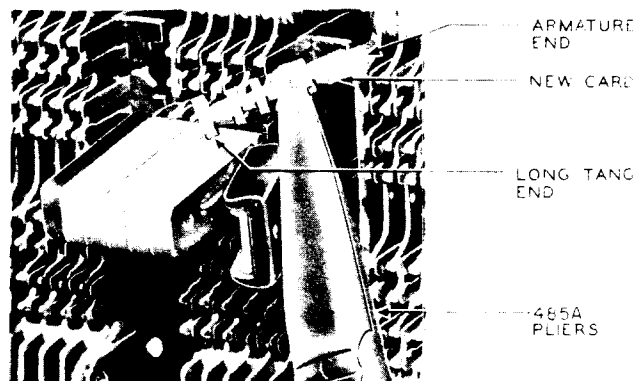
Fig. 10—Grasping a New Card for Replacement
