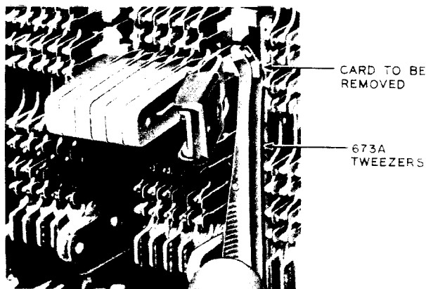
Fig. 9—Rotate Card to a Flat Position With Tweezers
