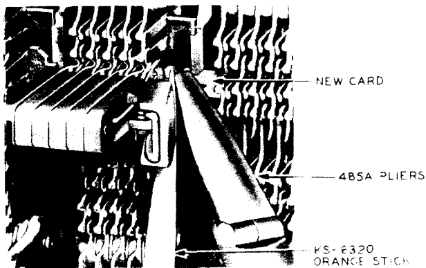
Fig. 11—Inserting New Card in Spring Combination
