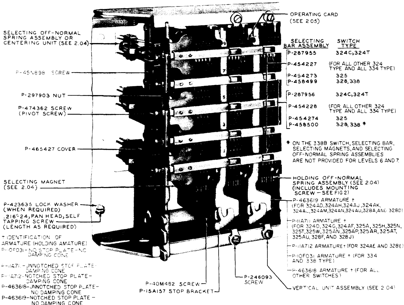
Fig. 1—Front View of Switch
