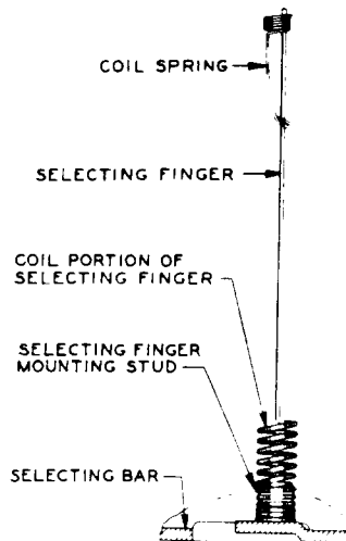
Fig. 4—Method of Assembling Coil Spring of Selecting Finger
