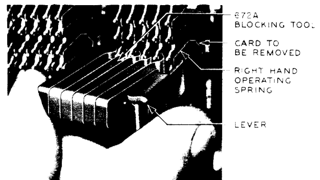
Fig. 7—Applying Blocking Tool
