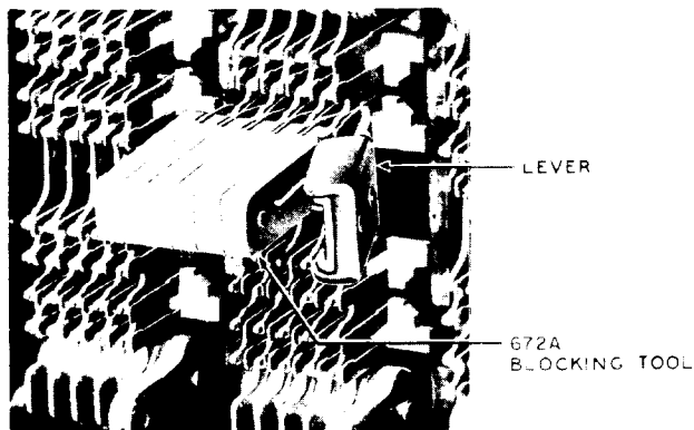
Fig. 8—Blocking Tool in Position
