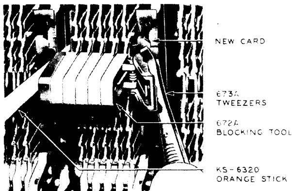
Fig. 12—Final Positioning Operations of New Card
