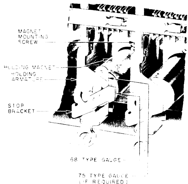
Fig. 5—Method of Determining Front Contact Make Gauging Value
