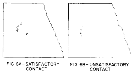
Fig. 6—Carbon Impressions of Contact Between Holding Armature and Holding Magnet Core Pole Face
