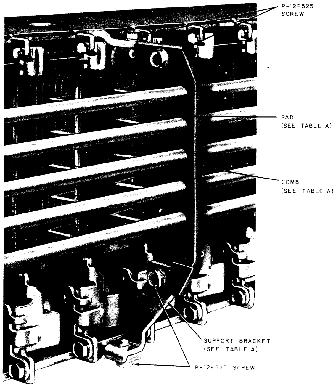
Fig. 2—Partial Front View of Switch Showing Comb and Support Bracket
