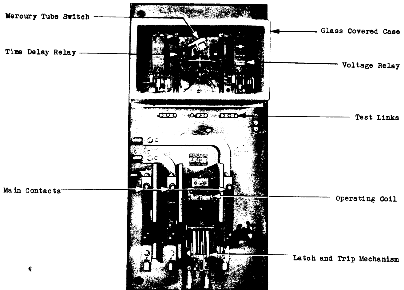
Fig. 1 - Master Switch (Without Cabinet)
