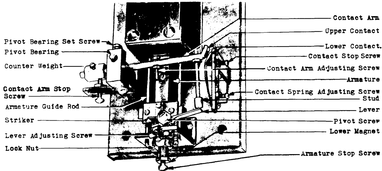
Fig. 3 - Voltage Relay Details
