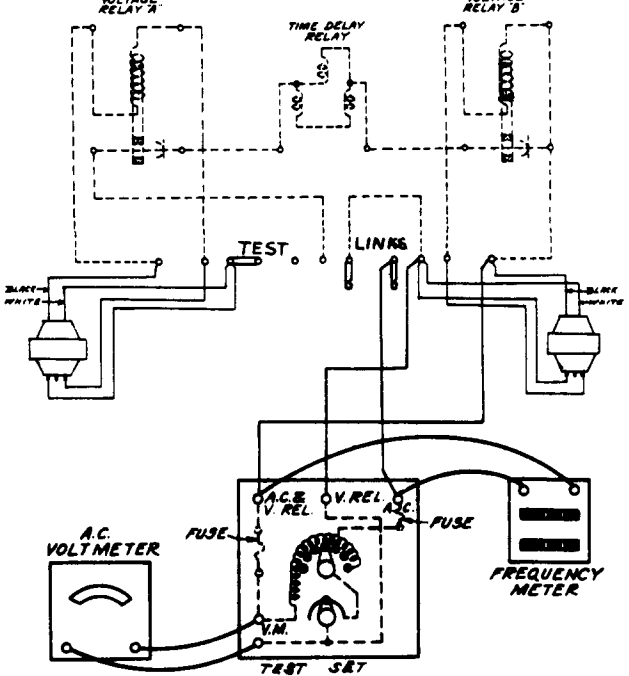
Fig. 9 - Test Connections for Relay "B" With Transformer
