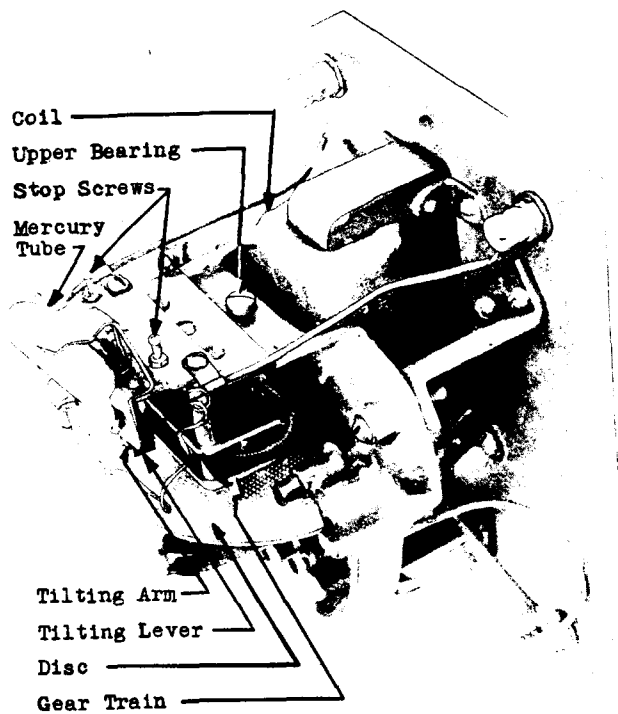
Fig. 4 - Time Delay Relay
