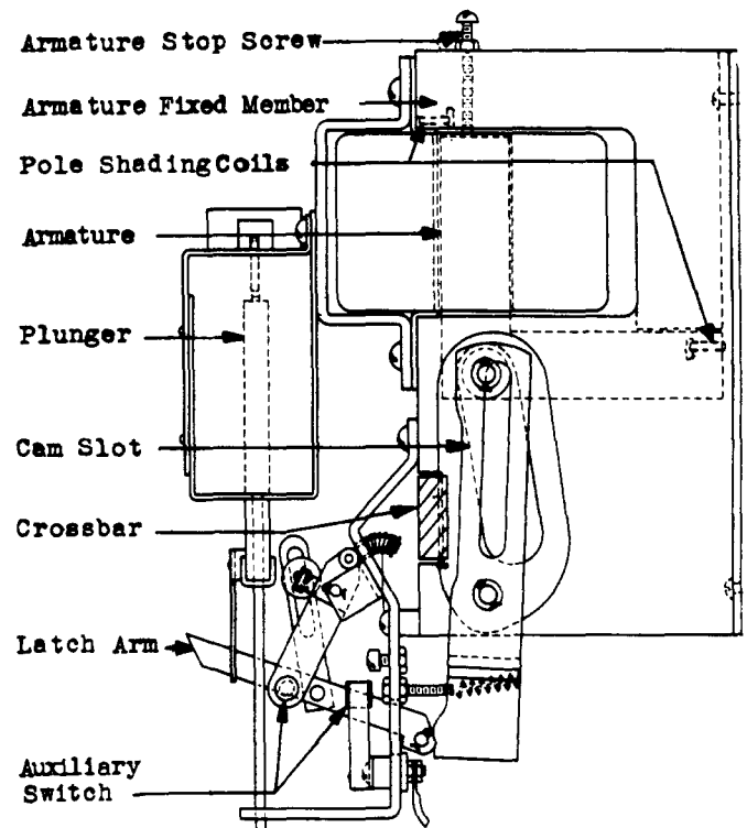
Fig. 12 - Operating, Tripping and Latch Mechanism
