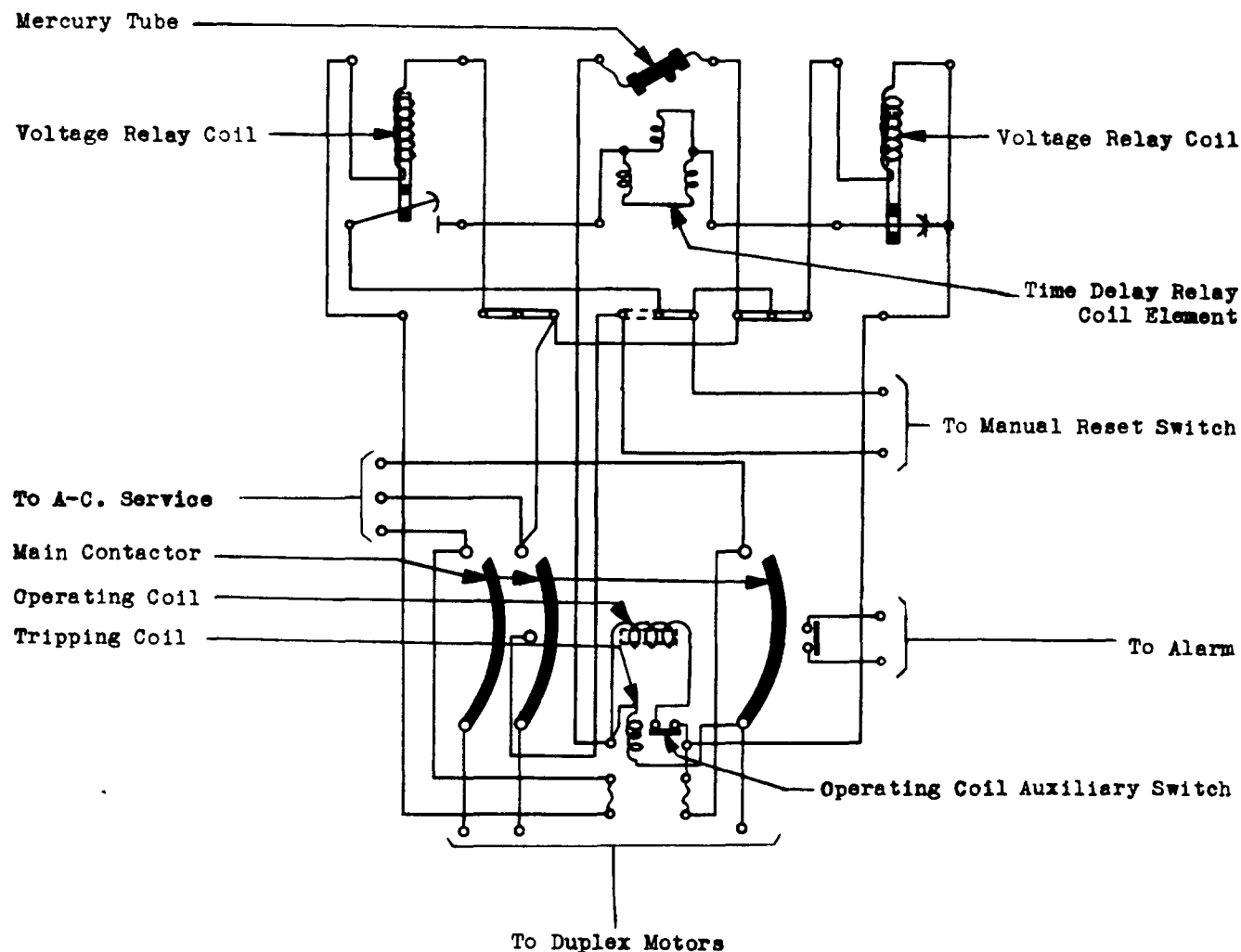
Fig. 2 - Circuit Schematic (Shown Without Transformers and Arranged for Manual Reclosing)
