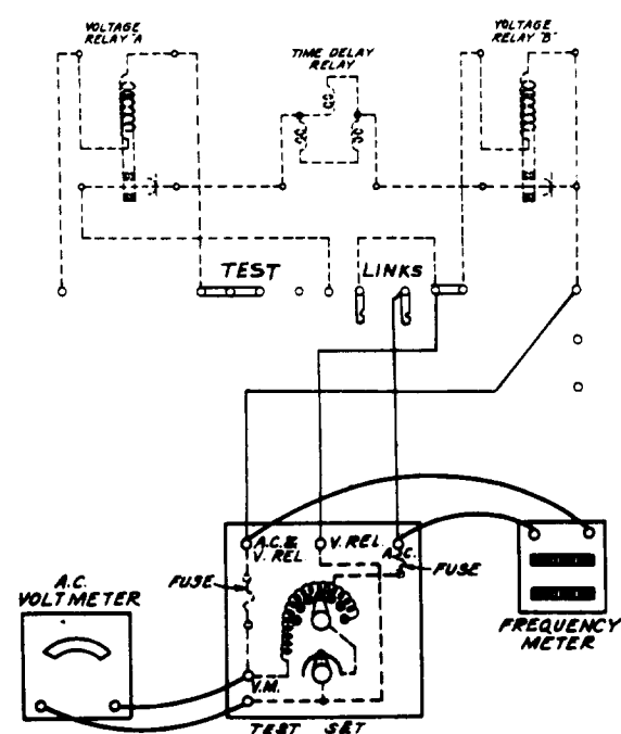
Fig. 7 - Test Connections for Relay "B" Without Transformer
