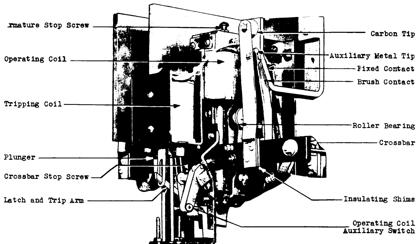
Fig. 5 – Contactor, Trip and Latch Mechanism
