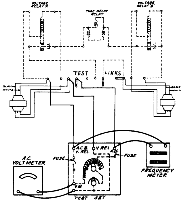
Fig. 8 - Test Connections for Relay "A" With Transformer
