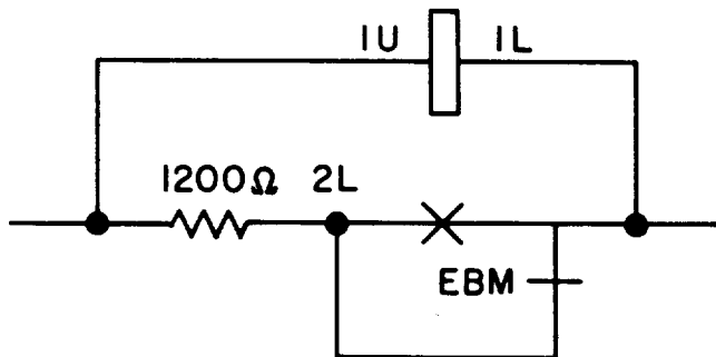
Fig. 3—Winding, Resistor, and Contact Arrangement
