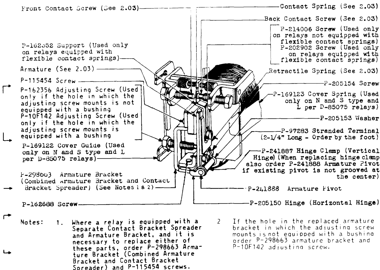
Fig. 2 - Designation of Parts — L-, N-, and S-Type Relays
