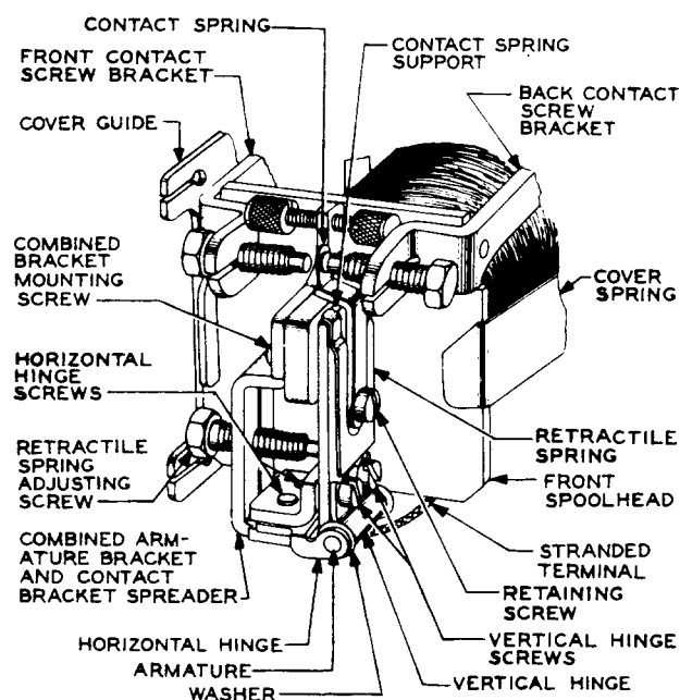
Fig. 3 – S-type Relay Equipped with Combined Armature Bracket and Contact Bracket Spreader
