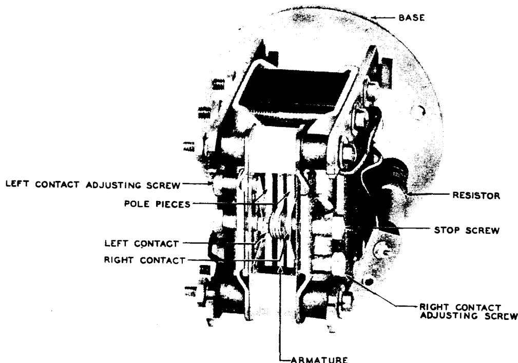
FIG. 1-KS-14499 RELAY
