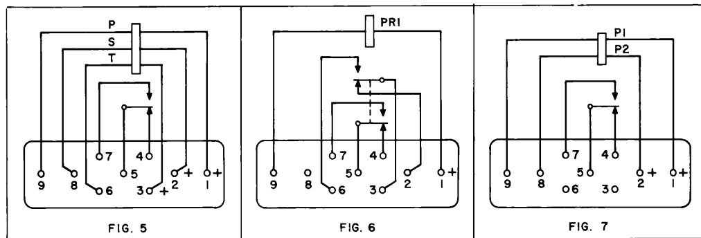
316-Type Relays
