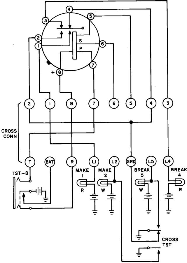
Fig. B — Cross-Connections When Testing 275- and 276-Type Relays Having BSP Fig. 8, Using Test Sets L1 and L2
