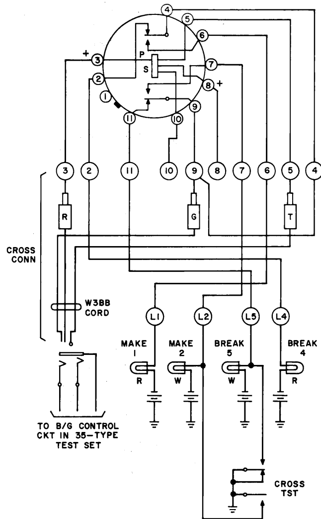
Fig. E — Cross-Connections When Testing 321-Type Relays Having BSP Fig. 1, Using Test Set L4
