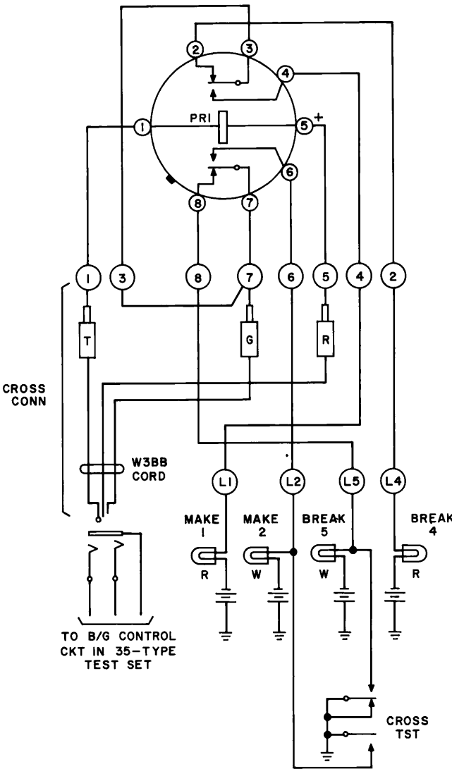
Fig. D — Cross-Connections When Testing 320-Type Relays Having BSP Fig. 1, Using Test Set L4
