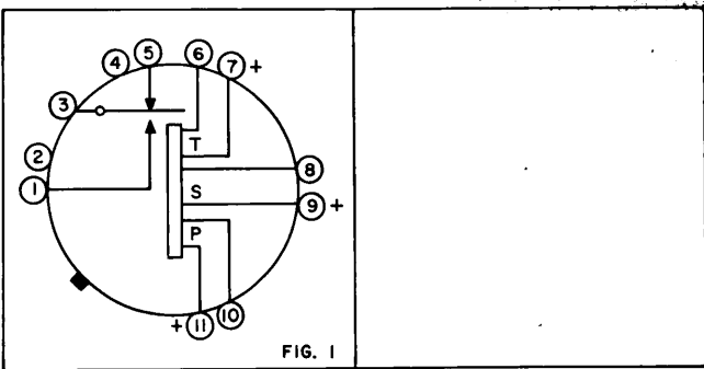
301-Type Relays
