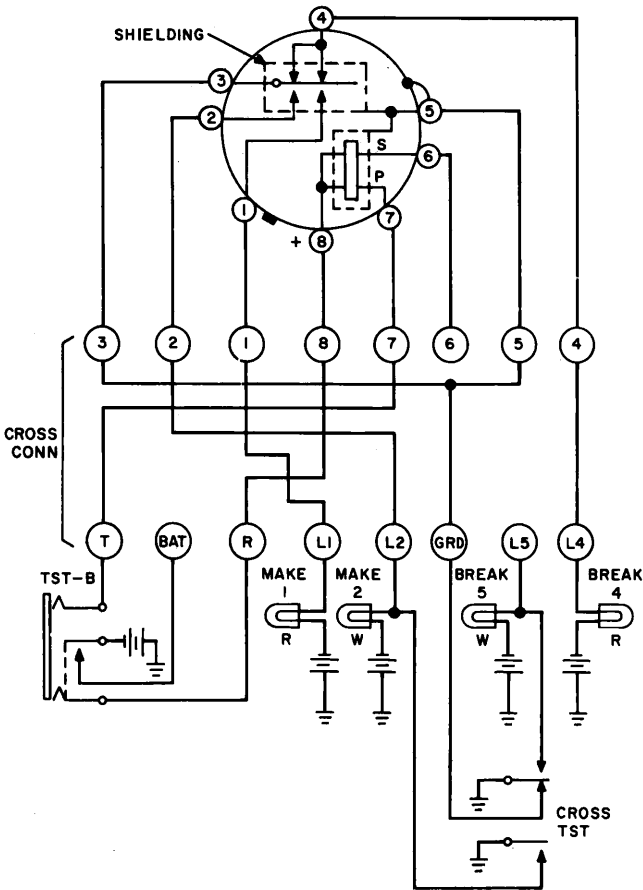
Fig. A — Cross-Connections When Testing 275- and 276-Type Relays Having BSP Fig. 6, Using Test Sets L1 and L2
