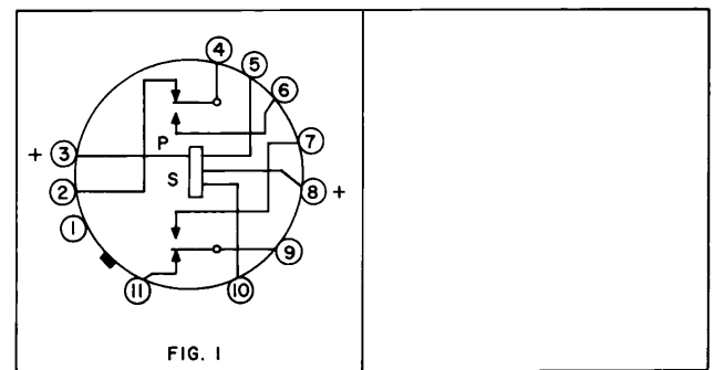
321-Type Relays
