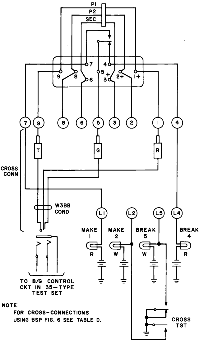
Fig. C — Cross-Connections When Testing 316-Type Relays Having BSP Fig. 1, 2, 3, 4, 5 or 7, Using Test Set L4
