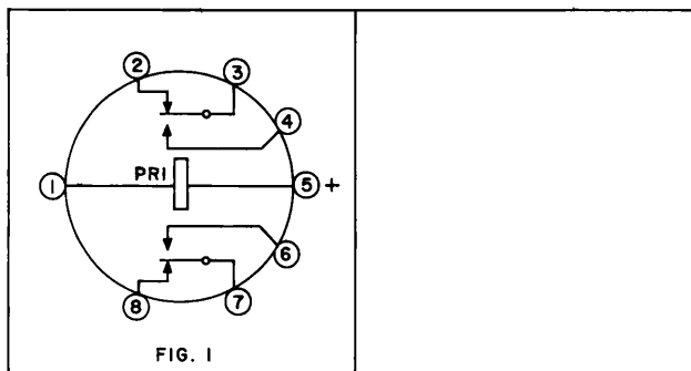
320-Type Relays
