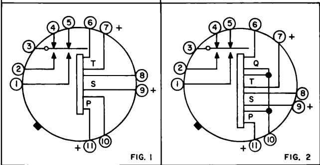
292-Type Relays
