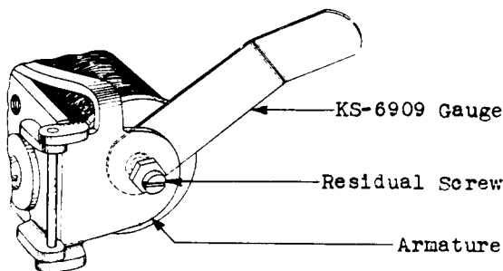
Fig. H — Checking the Residual Airgap
