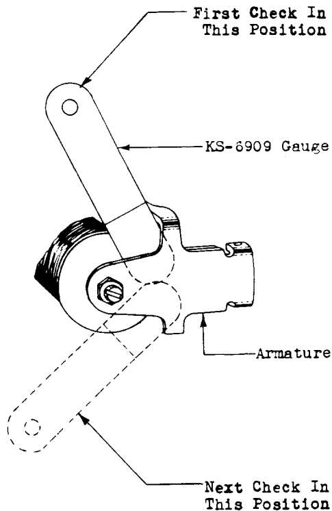
Fig. N — Checking Minimum Test, and Minimum and Maximum Readjust Heelpiece Airgap on 247- and 248-Type Relays
