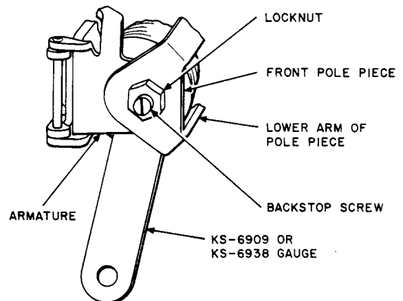
Fig. U—Checking Armature Travel and Spring Gauging on 251- and 252-Type Relays
