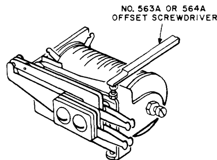
Fig. Y—Adjusting for Armature Movement
