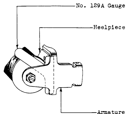
Fig. M — Checking Maximum Test Heelpiece Airgap on 247- and 248-Type Relays
