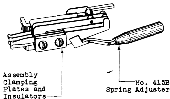
Fig. AH - Adjusting Spring to Meet the Spring Gauging Requirements
