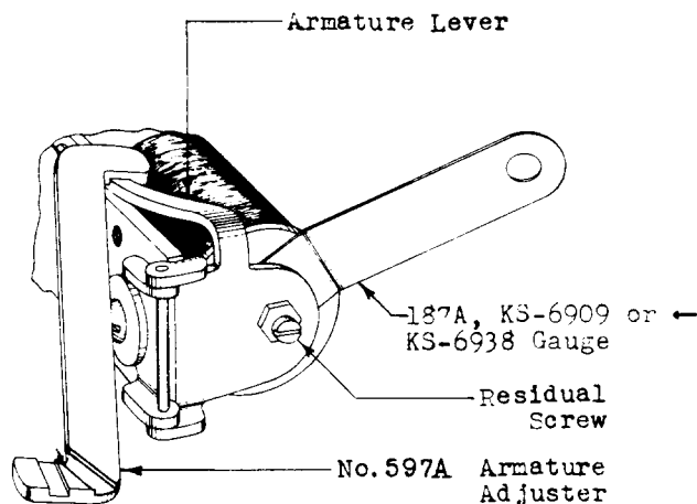
Fig. AC – Method of Adjusting the Armature Lever
