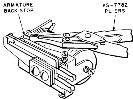
Fig. AE—Adjusting the Armature Stud Gap on Relays Equipped With Pivot-Type Armature
