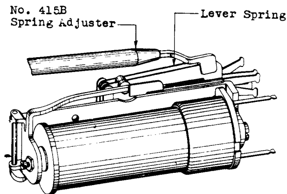
Fig. AF – Adjusting Lever Spring for Tension
