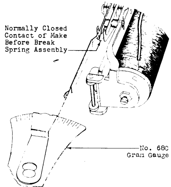
Fig. W — Measuring Contact Pressure on Make-Before-Break Spring Combination
