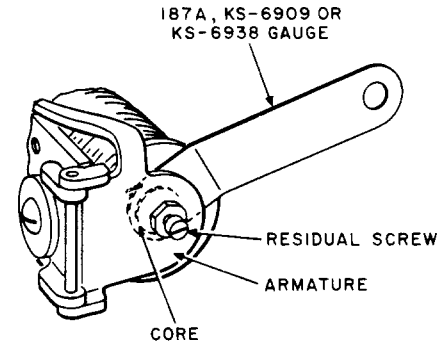
Fig. S—Checking Armature Travel and Spring Gauging on all Except 251- and 252-Type Relays Where Method Illustrated in Fig. R Cannot Be Applied
