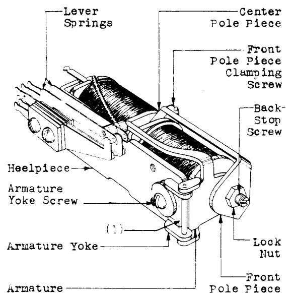
Fig. I — Heelpiece Airgap Requirement — 251-Type Relay Shown
