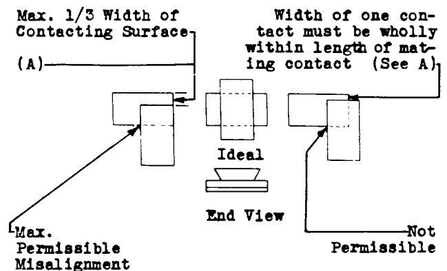
Fig. D — Alignment of Heavy Bar Contacts — Plan View of Contacting Surfaces
