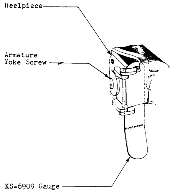
Fig. L — Checking Minimum Heelpiece Airgap on 221-, 222-, 251-, and 252-Type Relays
