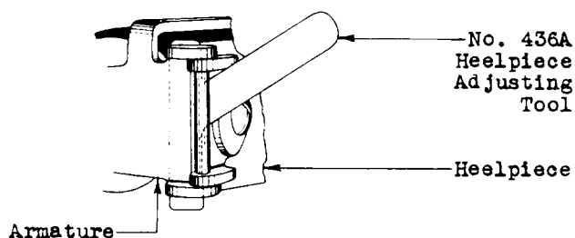
Fig. AA – Adjusting the Heelpiece Airgap With the No. 436A Heelpiece Adjusting Tool Inserted From the Heelpiece Side (all except the No. 223BN relay and 225-, 247-, and 248-type relays)
