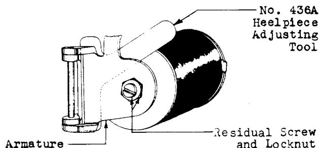
Fig. Z – Adjusting the Heelpiece Airgap With the No. 436A Heelpiece Adjusting Tool Inserted From the Armature Side (all except 251- and 252-type relays)
