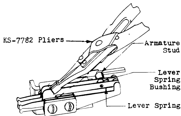
Fig. AG – Removing Excessive Bow From Spring
