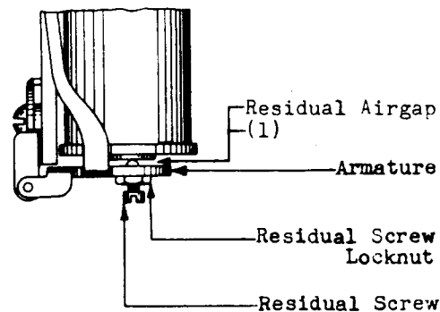
Fig. G - Illustrating Residual Airgap
