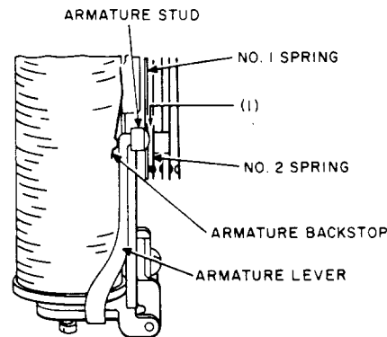
Fig. V—Illustrating Armature Stud Requirement
