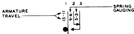
Fig. P — Typical Spring Combination Figure Showing Armature Travel and Spring Gauging Values
