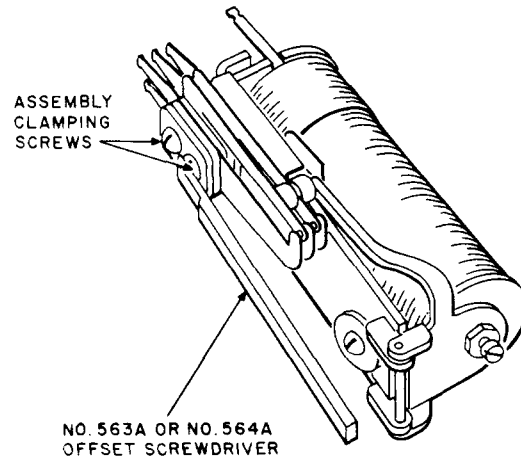
Fig. X—Aligning Contact Springs
