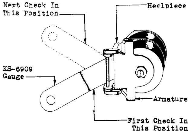
Fig. K — Checking Minimum and Maximum Heelpiece Airgap on 223- and 224-Type Relays and the Maximum Gap on 221-, 222-, 251-, and 252-Type Relays
