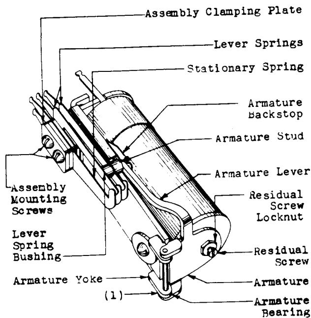
Fig. E - 221-Type Relay
