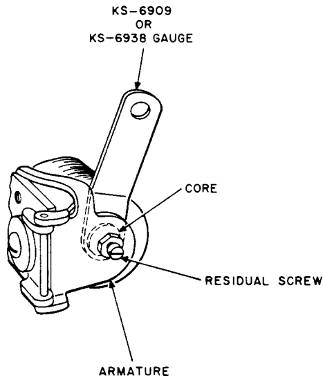
Fig. R—Checking Armature Travel and Spring Gauging On All Relays Except 251 and 252 Types
