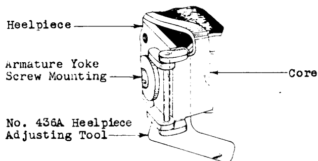
Fig. AB – Adjusting the Heelpiece Airgap on 251- and 252-Type Relays With the No. 436A Heelpiece Adjusting Tool Inserted From the Bottom
