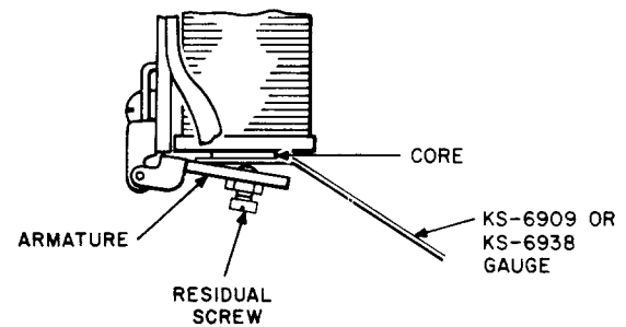
Fig. T—Incorrect Method of Checking Armature Travel and Spring Gauging
