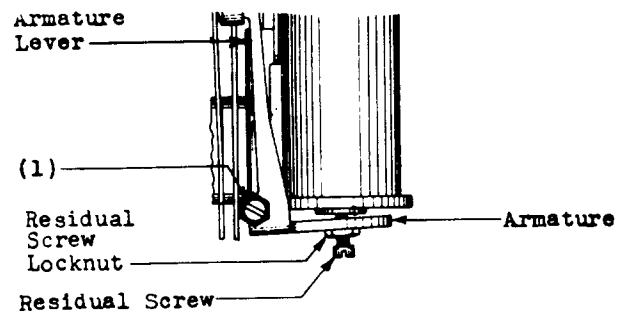
Fig. F - Illustrating Armature Movement Requirement for Pivot-Type Relays
