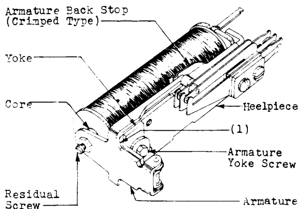
Fig. J — Heelpiece Airgap Requirement — 248-Type Relay Shown
