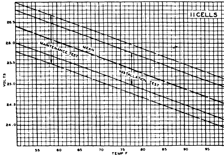
Fig. 5 - 253A Relay Operate Limits (Without Rheostat)
