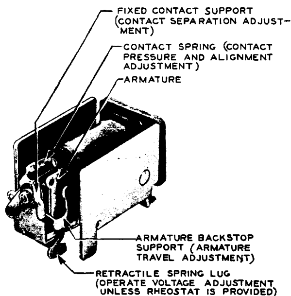
Fig. 1 - 253-Type Relay (End View All Types)
