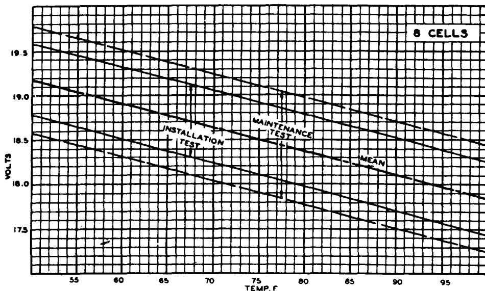
Fig. 4 - 253B Relay Operate Limits (Without Rheostat)
