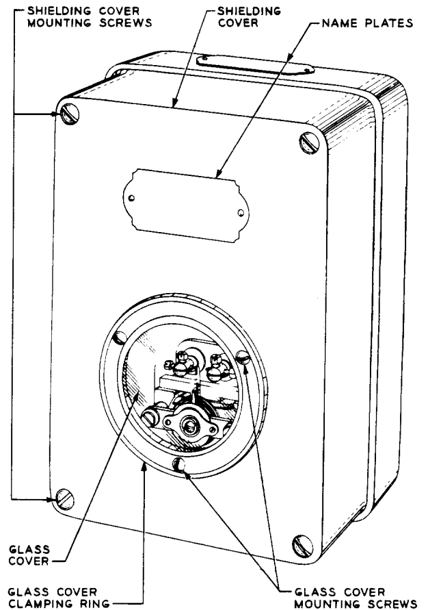
Fig. 8 - Weston Model 546
