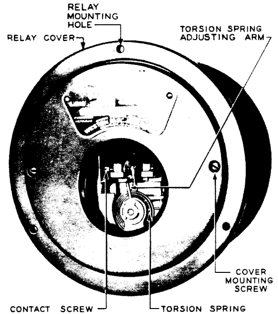
Fig. 7 - Weston Model 534 (flush mounting case)
