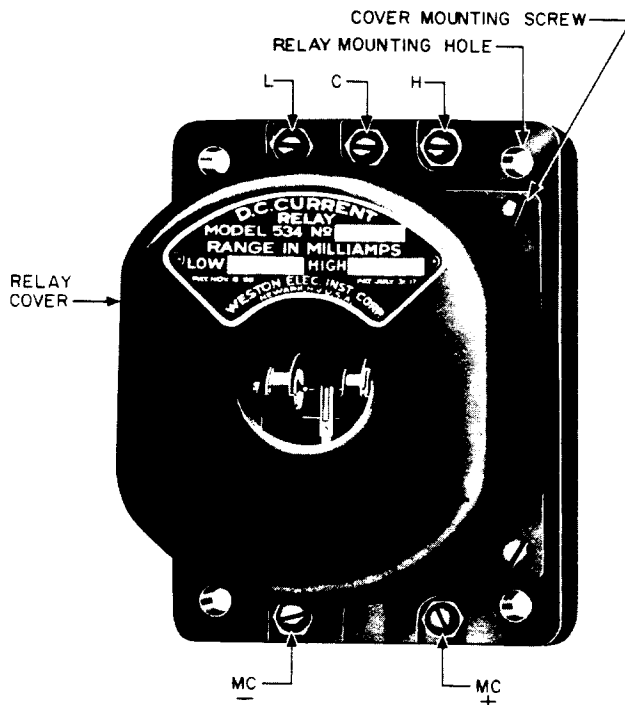
Fig. 6 - Weston Model 534 (surface case)
