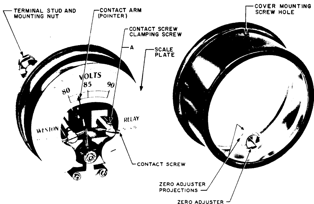
Fig. 10 — Model 730 (surface case) — Cover Removed — Used in Power Plants
