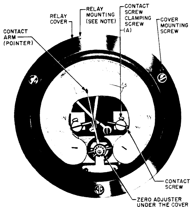
Fig. 9 — Model 730 (flush mounting case) — Front View
