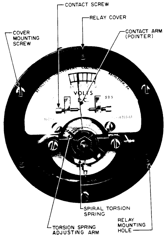
Fig. 12 — Bethlehem Model 1026 (flush mounting case) — Front View
