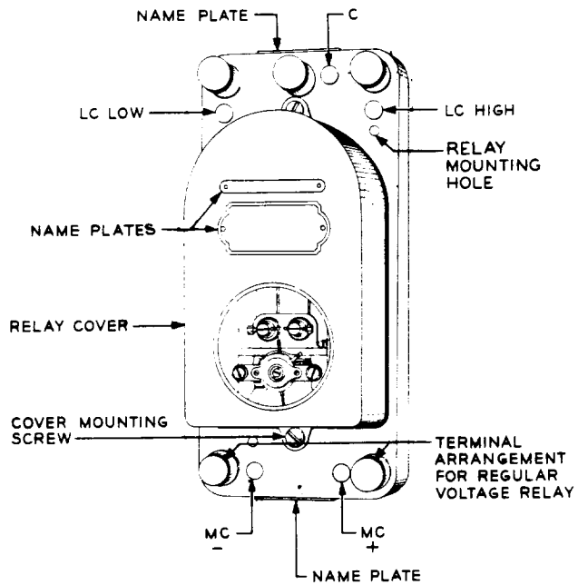
Fig. 5 - Weston Model 30
