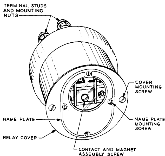
Fig. 1 - Western Electric 260 Type
