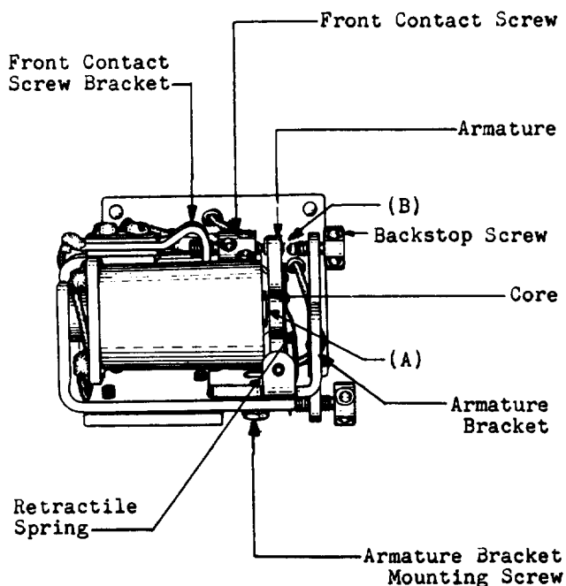
Fig. 4 — Front View — 268 Type Relay
