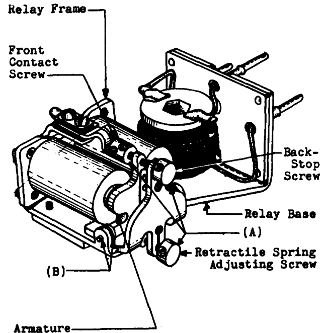
Fig. 1 — General View — 268A Relay
