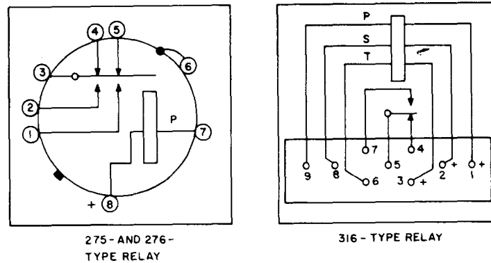
Fig. 5—Winding and Contact Arrangements
