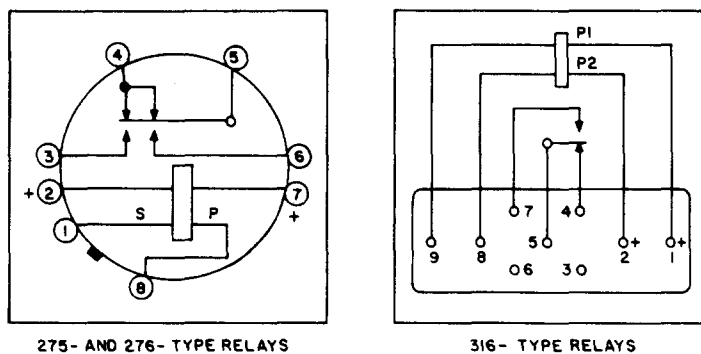
Fig. 7—Winding and Contact Arrangements
