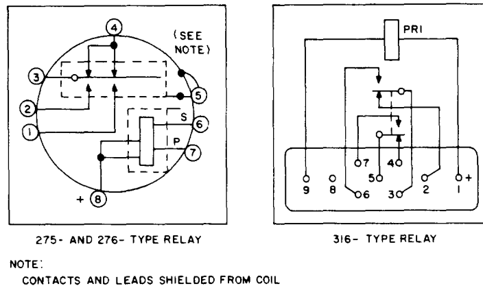
Fig. 6—Winding and Contact Arrangements
