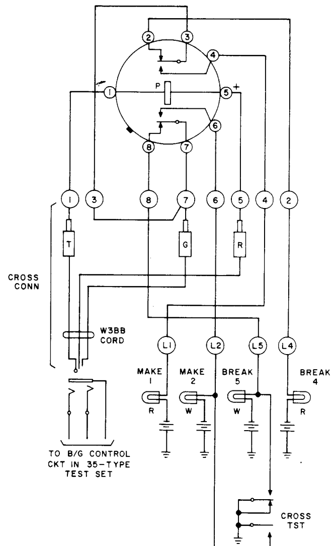
Fig. 13—Cross-Connections Testing 320-Type Relays, Shown in Fig. 1, Using Test Set L4
