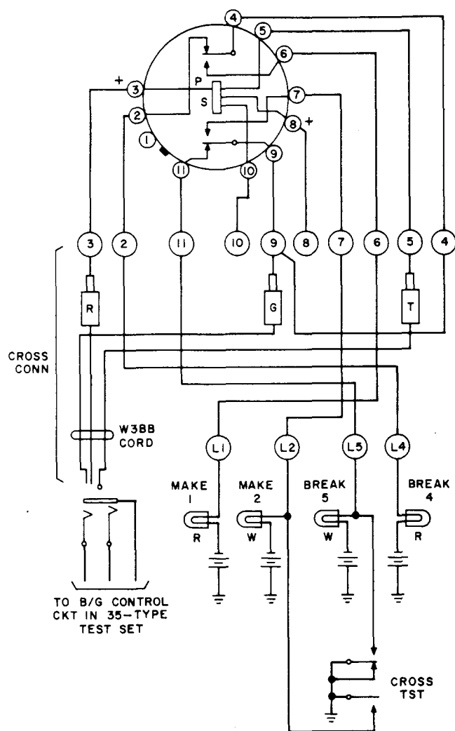
Fig. 14—Cross-Connections When Testing 321-Type Relays, Shown in Fig. 1, Using Test Set L4
