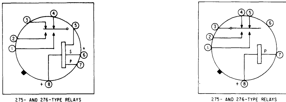
Fig. 8—Winding and Contact Arrangements
