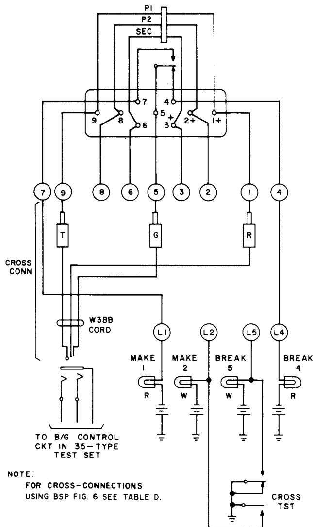
Fig. 12—Cross-Connections When Testing 316-Type Relays, Shown in Fig. 1, 2, 3, 4, 5, or 7, Using Test Set L4
