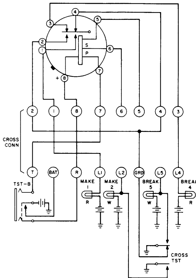
Fig. 11—Cross-Connection When Testing 275- and 276-Type Relays, Shown in Fig. 8, Using Test Sets L1 and L2
