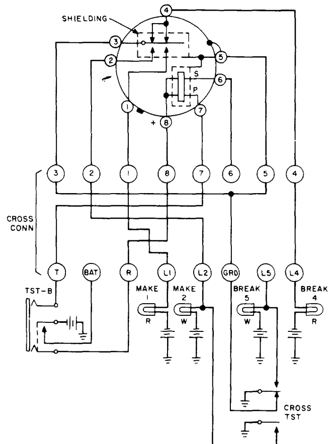
Fig. 10—Cross-Connections When Testing 275- and 276-Type Relays, Shown in Fig. 6, Using Test Set L1 and L2
