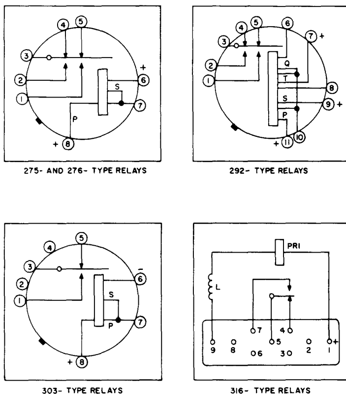
Fig. 2—Winding and Contact Arrangements
