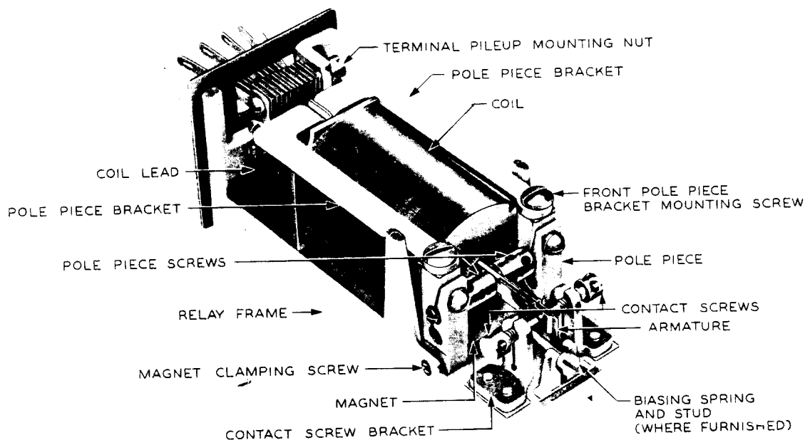
Fig. 5 - 280-Type Relay — General View With Shell and Cover Cap Removed
