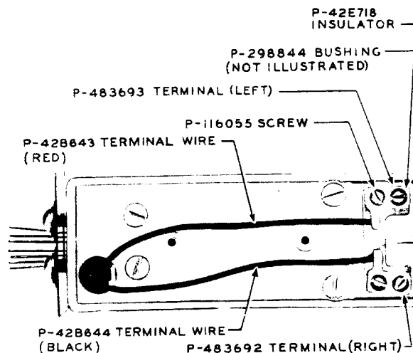
Fig. 3 - 280-Type Relay — Bottom View With Shell and Cover Cap Removed
