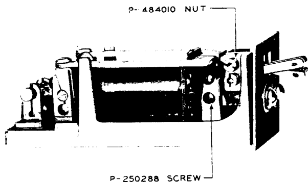
Fig. 2 - 280-Type Relay — Side View With Shell and Cover Cap Removed
