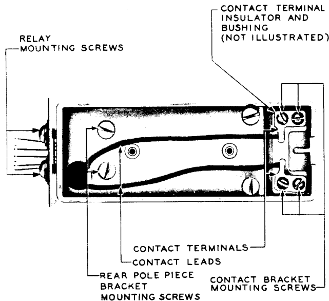
Fig. 6 - 280-Type Relay — Bottom View With Shell and Cover Cap Removed
