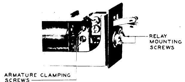
Fig. 7 - 280-Type Relay — Partial Side View With Shell and Cover Cap Removed
