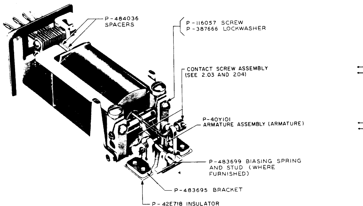
Fig. 4 - 280-Type Relay — General View With Shell and Cover Cap Removed
