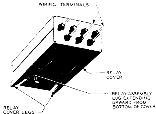
Fig. 2 - 289-Type Relay
