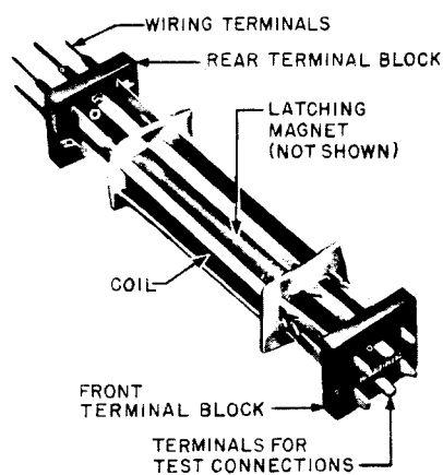
FIG.13B-LATCHING UNIT
