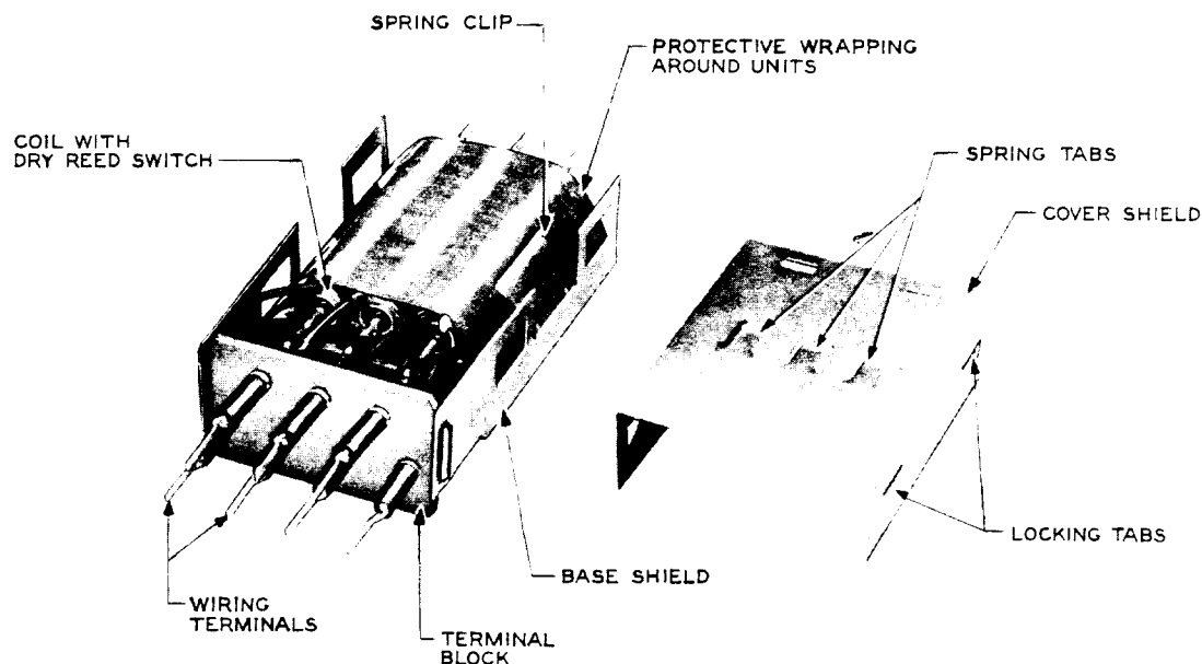
Fig. 3 - 289-Type Relay With Cover and Cover Shield Removed (bottom view)
