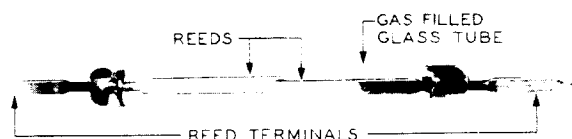
Fig. 1 — Sealed Contacts
