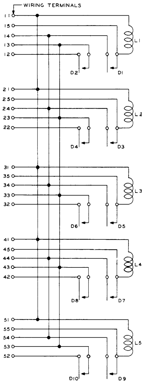
L1 TO L5 REPRESENT COILS OF INDIVIDUAL UNITS (5) IN RELAY. D1-D2; D3-D4; D5-D6; D7-D8; D9-D10 REPRESENT THE CONTACTS OF THE PAIR OF DRY REED SWITCHES IN THE INDIVIDUAL UNITS OF THE RELAY.
