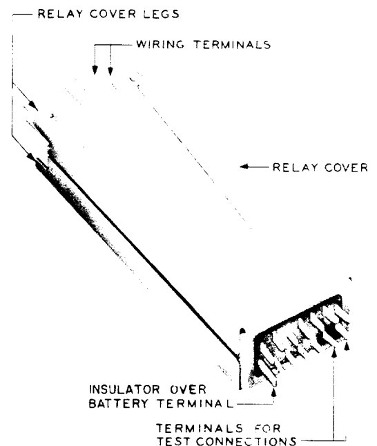
Fig. 11 – 295-Type Relay
