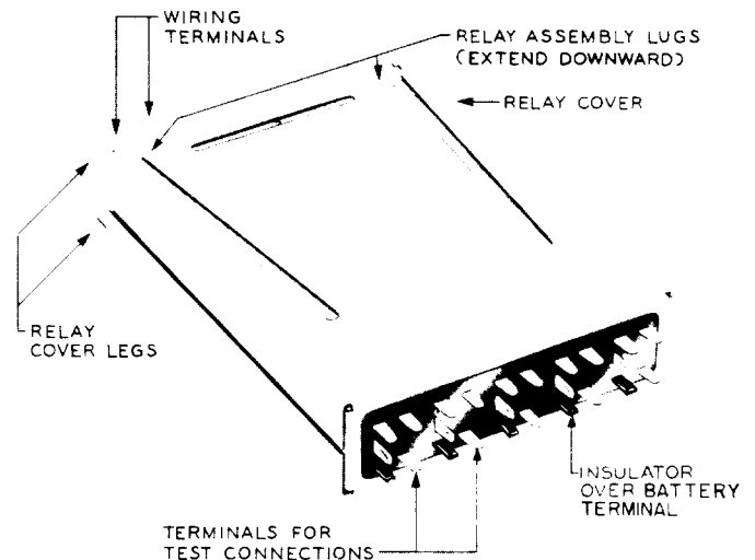
Fig. 7 - 293-Type Relay
