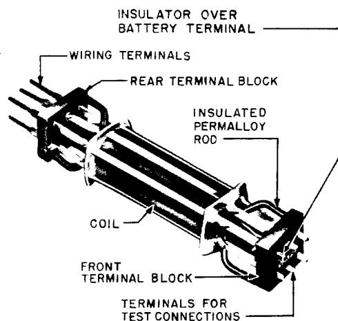
FIG 13A-NON LATCHING UNIT
