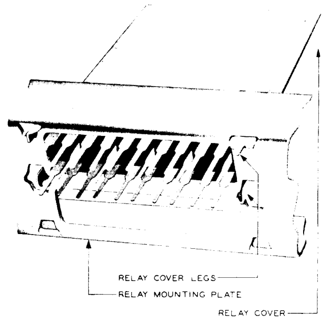
Fig. 10 – Mounting of 293-Type Relay
