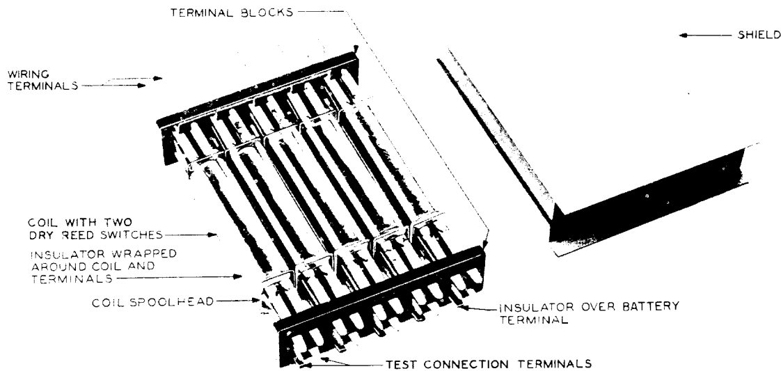
Fig. 8 - 293-Type Relay With Cover and Shield Removed
