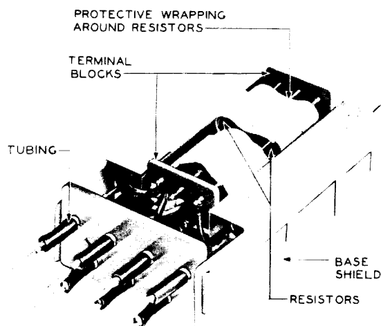
Fig. 4 - 289-Type Relay With Cover and Cover Shield Removed (top view)
