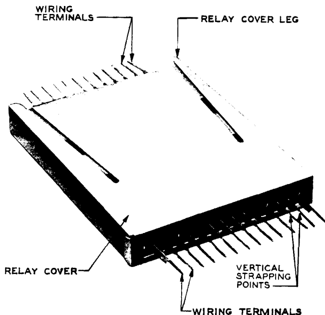
Fig. 5 - 290-Type Relay
