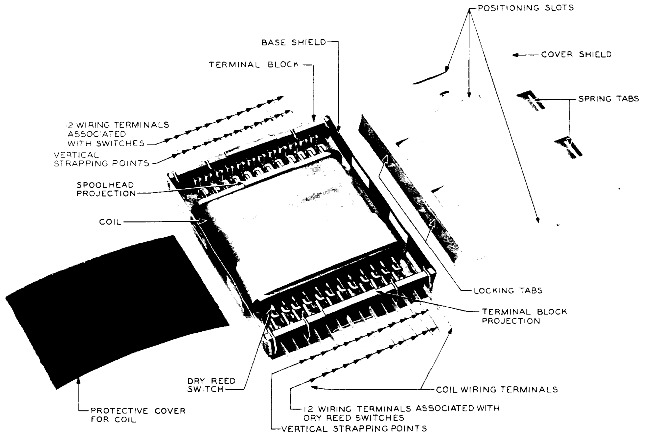
Fig. 6 - 290-Type Relay With Cover and Cover Shield Removed
