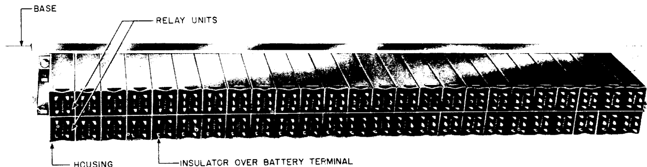
Fig. 12 - 302-Type Relay
