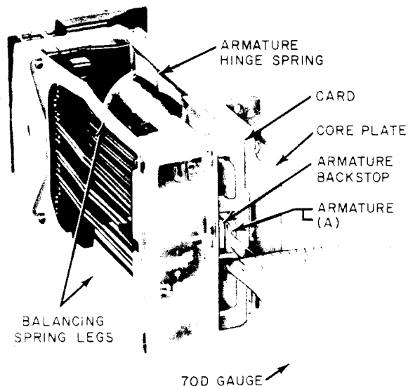
Fig. 4—Method of Checking Armature Back Tension—AF-Type Relay Illustrated
