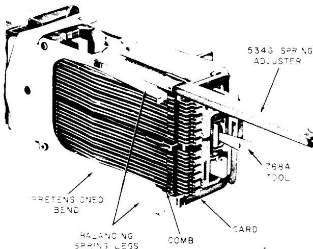
Fig. 11—Method of Adjusting Balancing Spring Tension
