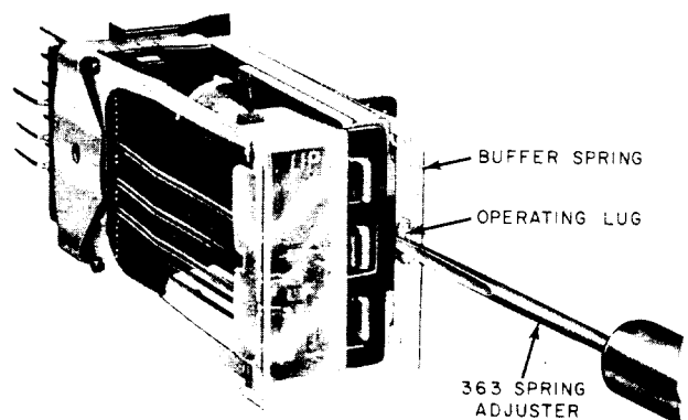
Fig. 13—Method of Positioning Buffer Spring
