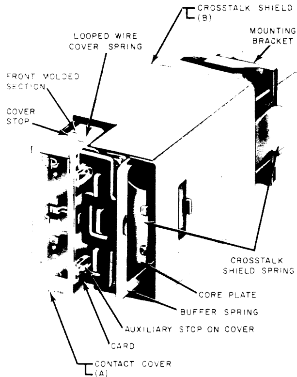
Fig. 1—AJ-Type 12-Position Relay With Cross-Talk Shield—Buffer Spring Positioned by Spoolhead—Wire Cover Spring and Contact Cover Without Metal Frame
