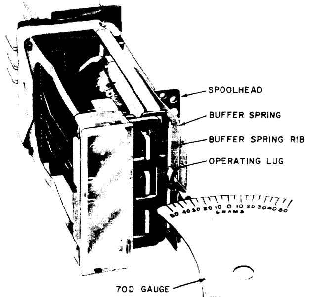
Fig. 8—Method of Checking Buffer Spring Tension (buffer spring positioned by spoolhead, illustrated)
