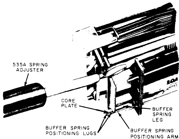
Fig. 15—Method of Adjusting Buffer Spring Tension—Buffer Spring Positioned by Core Plate
