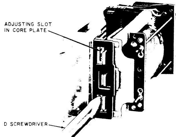
Fig. 12—Method of Adjusting Contact Separation
