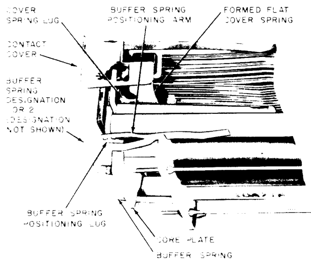
Fig. 2—AJ-Type 12-Position Relay—Buffer Spring Positioned by Core Plate—Flat Cover Spring and Contact Cover Without Metal Frame
