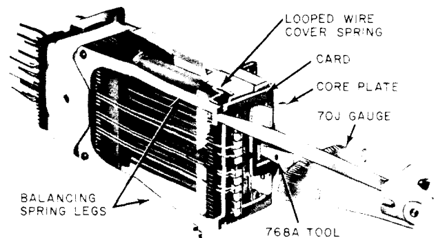
Fig. 9—Method of Removing Balancing Spring Legs from Cards
