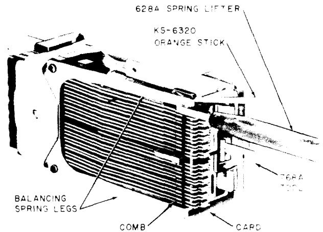
Fig. 9—Method of Removing Balancing Spring Legs from Cards
