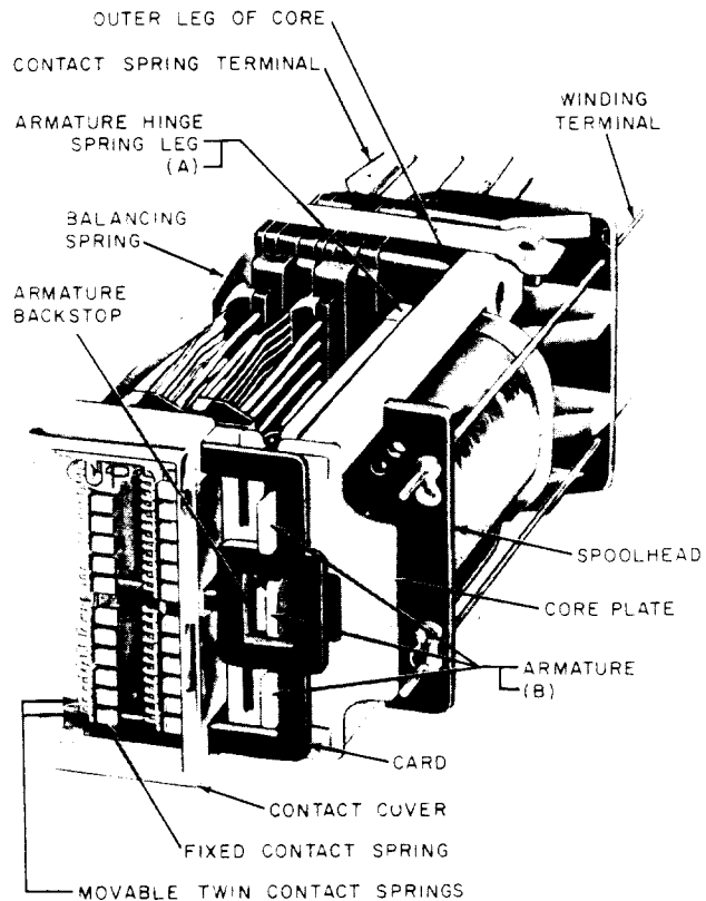
Fig. 3—AJ-Type 24-Position Relay
