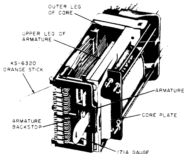
Fig. 6—Method of Checking Open or Closed Contacts
