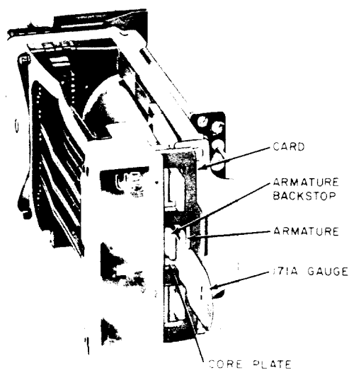
Fig. 7—Gauge Inserted Between Armature and Armature Backstop
