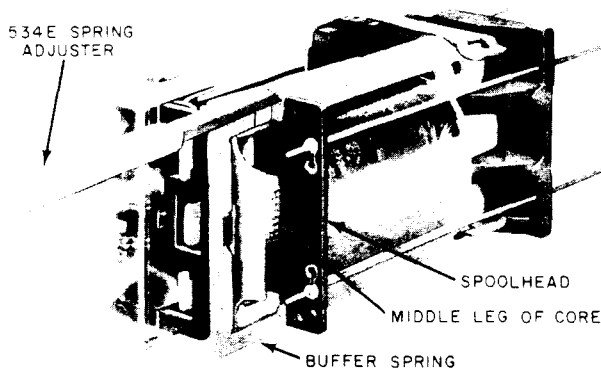
Fig. 14—Method of Adjusting Buffer Spring Tension—Buffer Spring Positioned by Spoolhead
