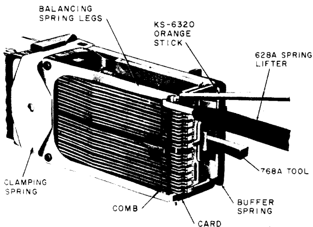
Fig. 6—Disengaging Balancing Spring From Card
