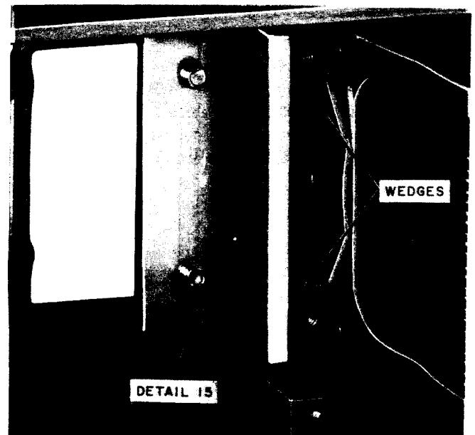
Fig. 21—Detail 15 Wedging Bracket in Place
