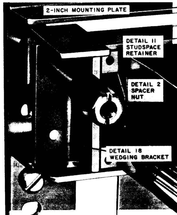
Fig. 14—Detail 18 Wedging Bracket in Place Over Left Detail 4 Stud
