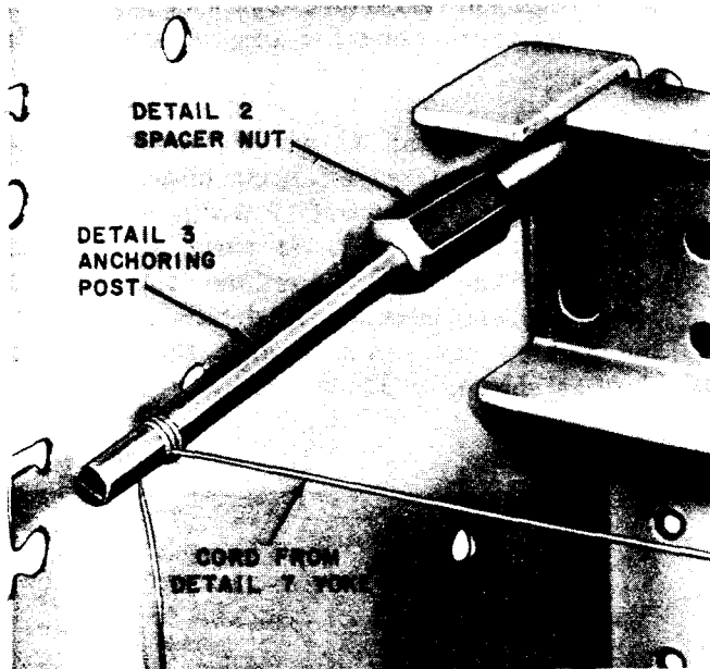
Fig. 16—Detail 3 Anchoring Post Inserted in Left Detail 2 Spacer Nut
