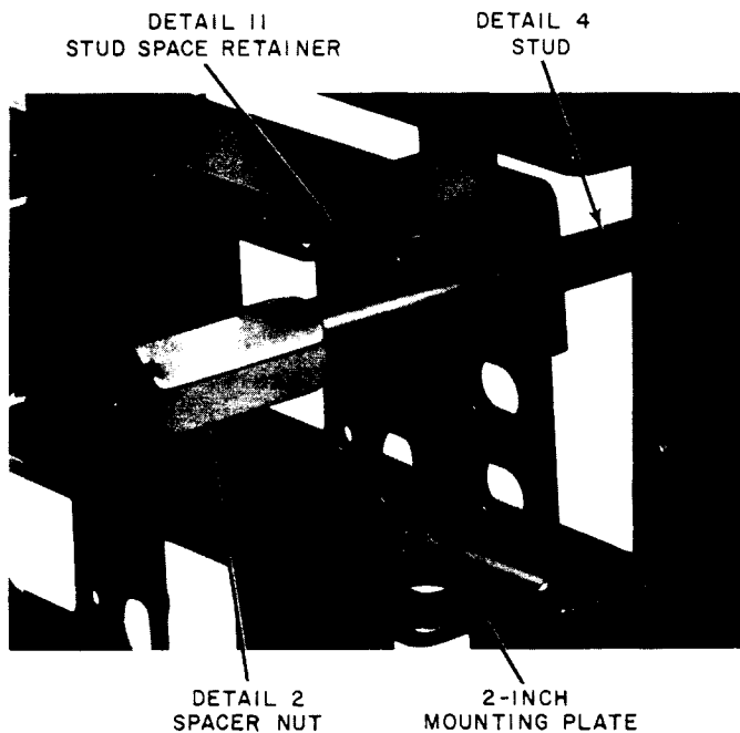
Fig. 13—Detail 4 Stud in Place With Detail 11 Stud Space Retainers
