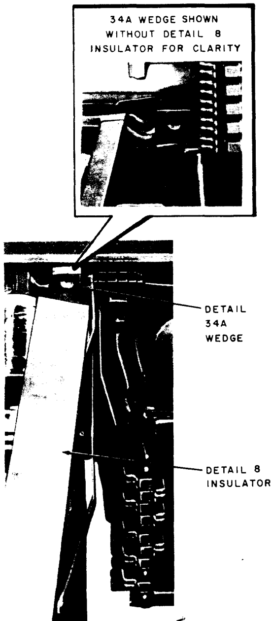
Fig. 17—Details 34A and 34B Wedges in Place With Detail 8 Insulators (34B Not Shown)
