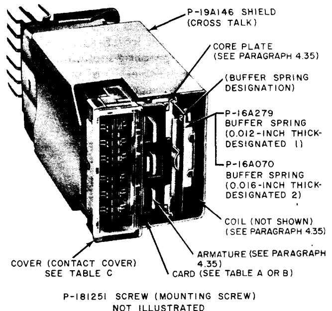
Fig. 1—12-Position Relay—General View
