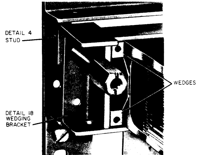
Fig. 20—Detail 18 Wedging Support on Detail 4 Stud
