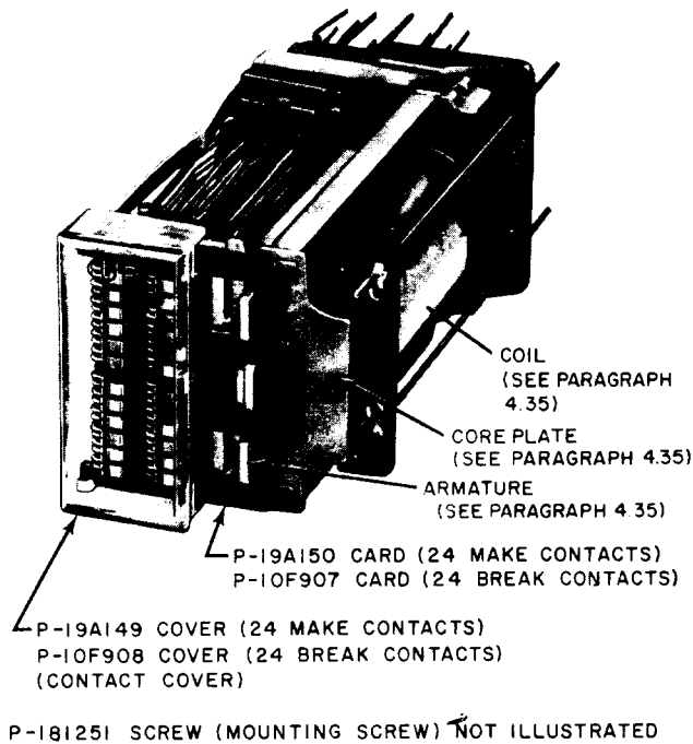
Fig. 2—24-Position Relay—General View
