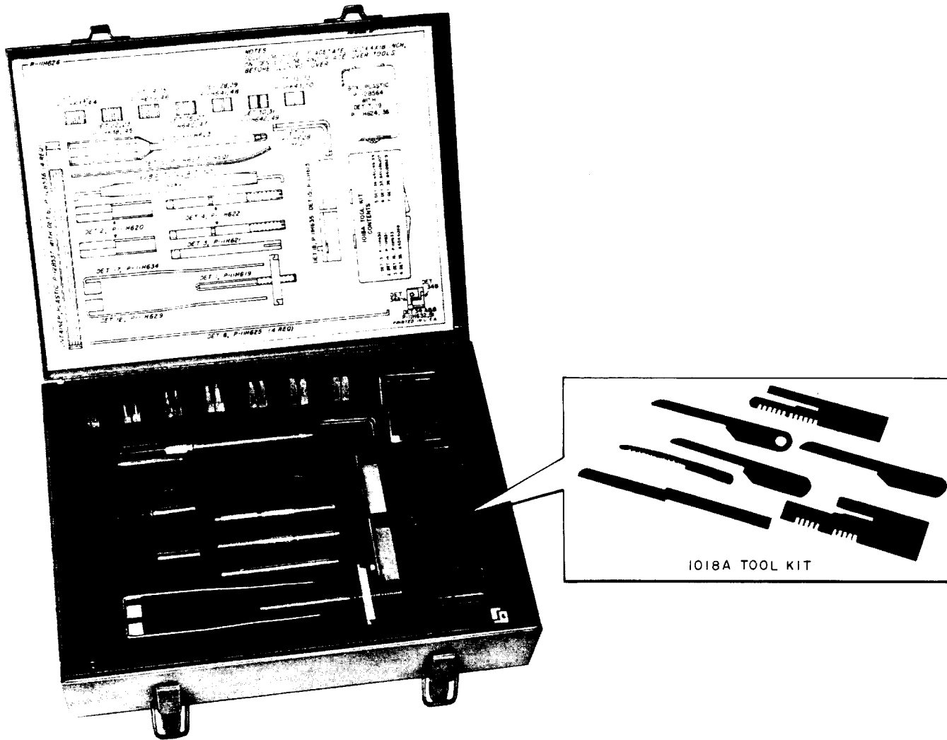
Fig. 3—1017A Tool Kit Including 1018A Tool Kit
