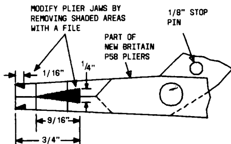
Fig. 4—Modification of New Britain P58 Pliers for Clip Removal
