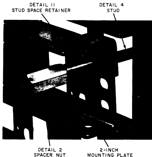
Fig. 12—Detail 4 Studs in Place With Detail 11 Stud Space Retainers
