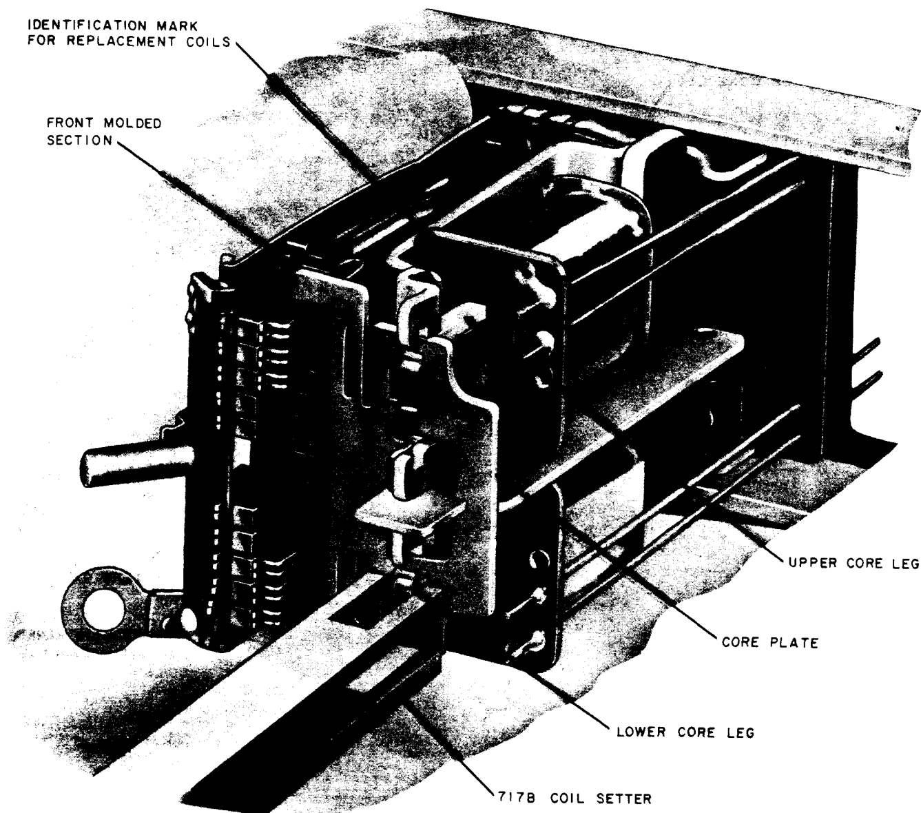
Fig. 35—Positioning Core Plate With 717B Coil Setter
