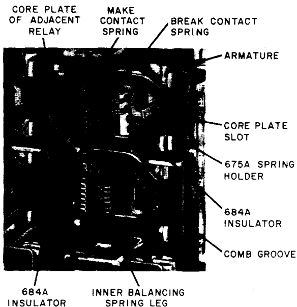
Fig. 27—684A Insulators and 675A Spring Holder Mounted on Upper Half of Relay
