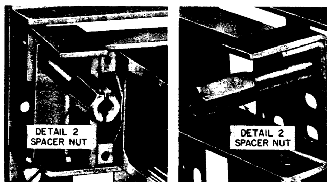
Fig. 14—Detail 2 Spacer Nuts in Place
