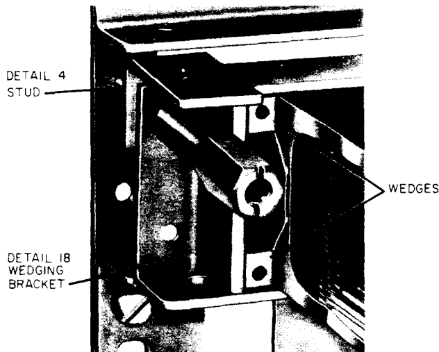
Fig. 19—Detail 18 Wedging Support on Detail 4 Stud
