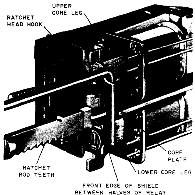
Fig. 31—Removing Core Plate
