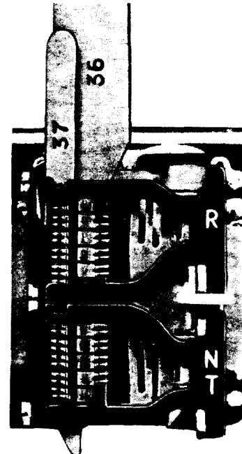
Fig. 7—Detail 37 Comb in Place With Detail 36 Lifter
