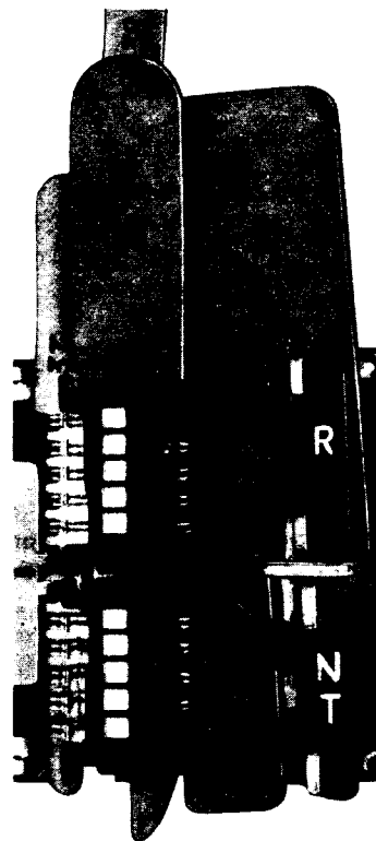
Fig. 10—Detail 16 Lifter in Place With Detail 14 Comb, Detail 37 Comb, and Detail 38 Comb Lifter
