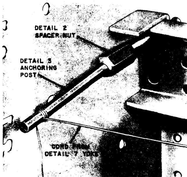
Fig. 15—Detail 3 Anchoring Post Inserted in Left Detail 2 Spacer Nut
