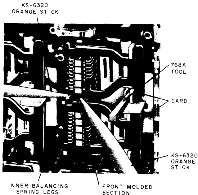
Fig. 5—Disengaging Inner Balancing Spring Leg From Upper Card
