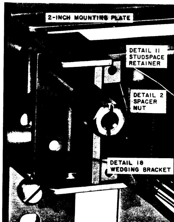
Fig. 13—Detail 18 Wedging Bracket in Place Over Left Detail 4 Stud
