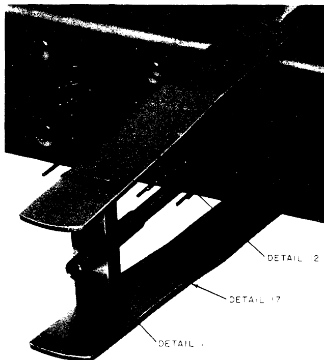
Fig. 17—Detail 12 Wedge Support, Detail 17 Wedge Support, and Detail 1 Wedge Support Assembly
