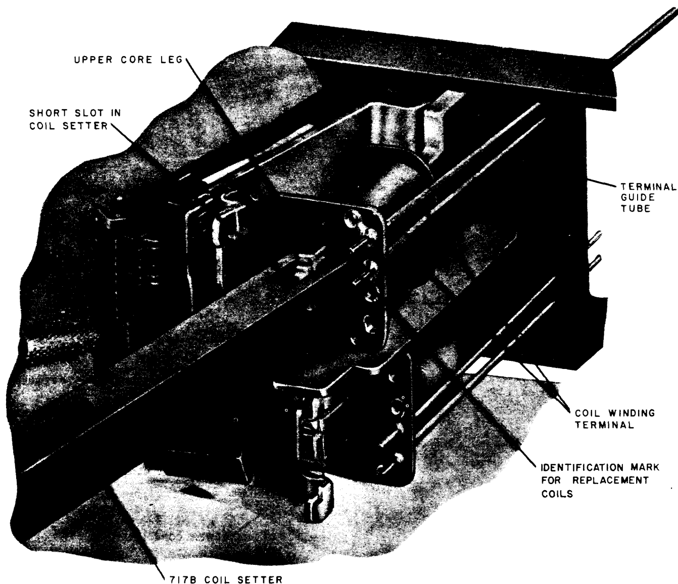
Fig. 34—Positioning Replacement Coil With 717B Coil Setter
