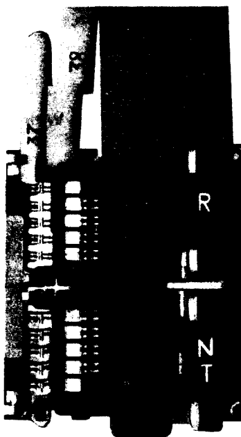
Fig. 9—Detail 14 Comb in Place With Detail 37 Comb and Detail 38 Comb Lifter
