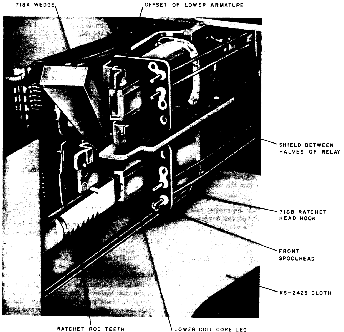
Fig. 33—Removing Lower Card
