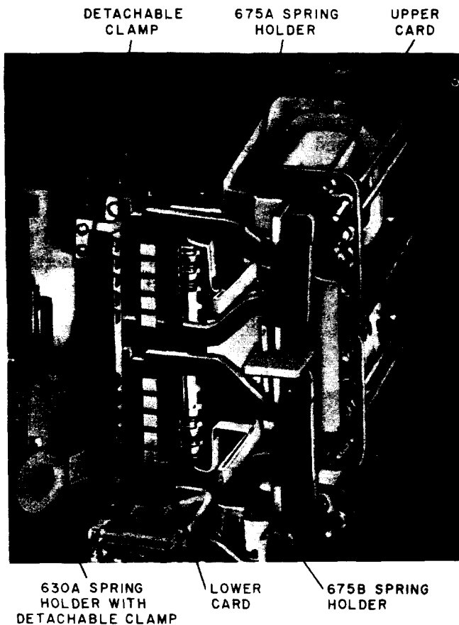
Fig. 30—Card Removal Tools Mounted in Place
