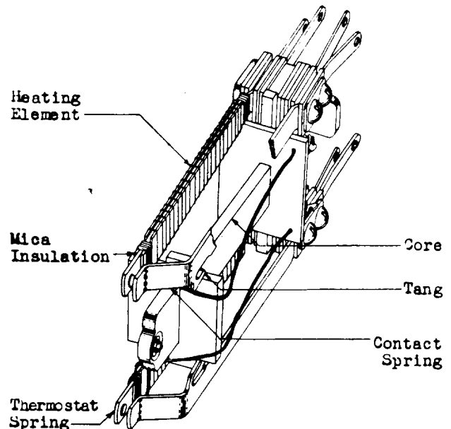
Fig. 1 - Relay Assembly (Cover Removed)
