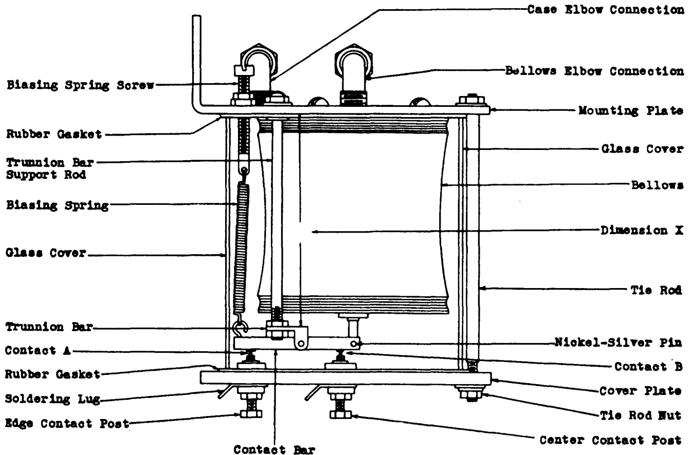
Fig. 1 - Assembly of Relay
