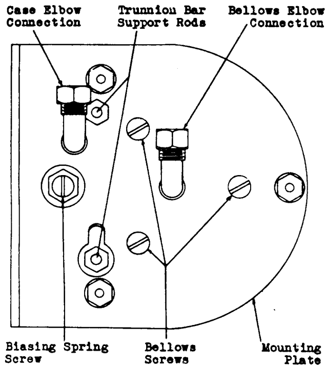
Fig. 4 - Top View of Relay
