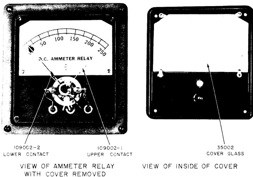
Fig. 2—KS-15802 Ammeter Relay
