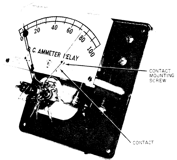
Fig. 5—Ammeter Relay Removed from Case
