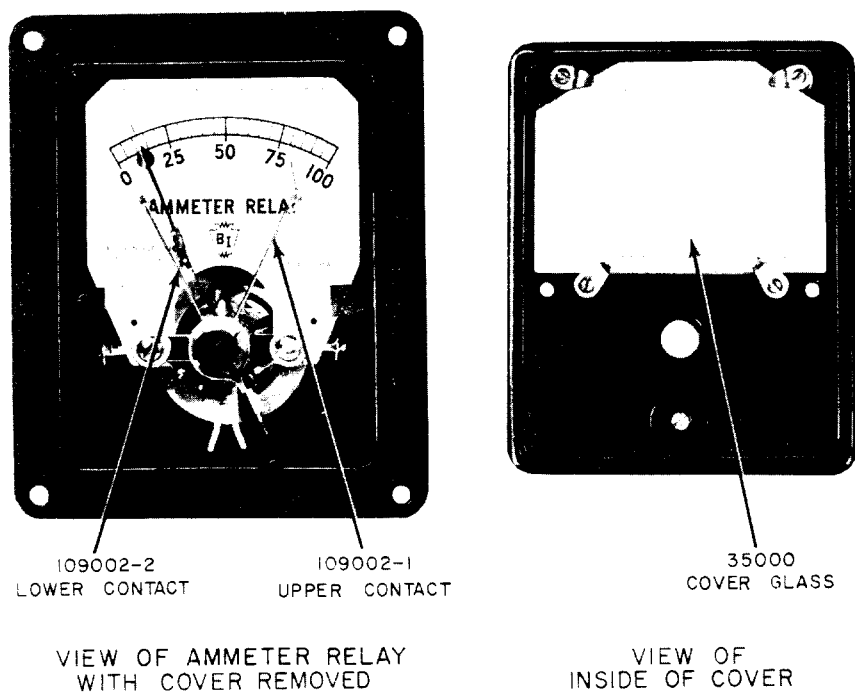
Fig. 3—KS-15803 Ammeter Relay
