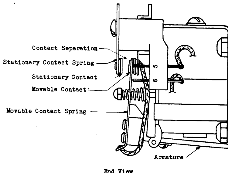
Fig. 1 - KS-5658 Relay
