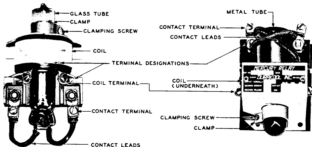
FIG. 1 - KS - 5721 RELAYS
