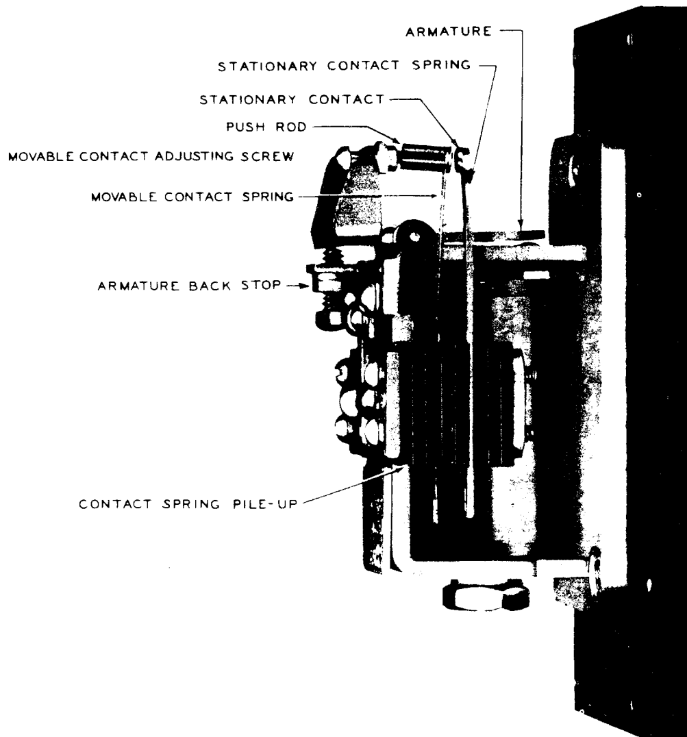
Fig. 1 - KS-13767 Relay
