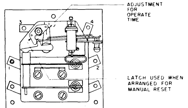
Fig. 1 - KS-15518 Relay
