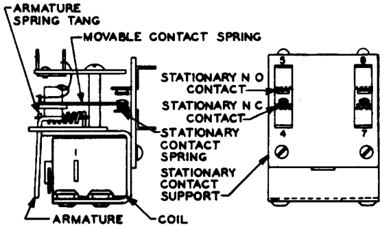
Fig. 2 - KS-15756 Relay
