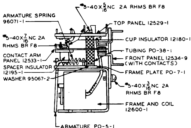
Fig. 1 - KS-15528 Relay
