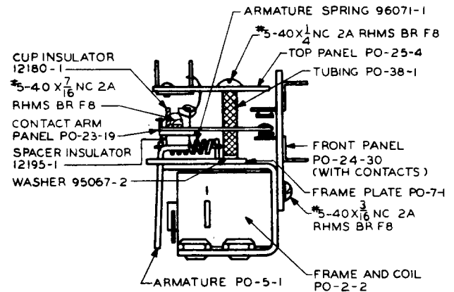
Fig. 2 - KS-15756 Relay
