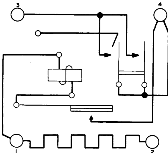
Fig. 2 - Schematic Diagram KS-15623 Relay
