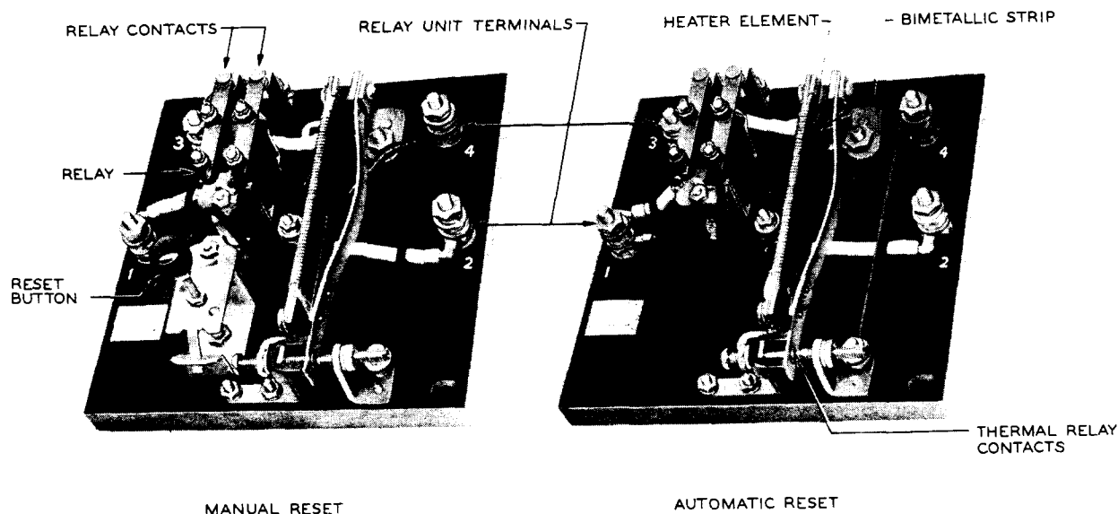
FIG. 1- TYPICAL KS-15623 RELAYS
