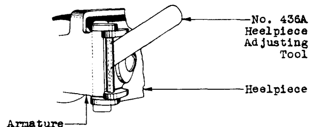
Fig. 24 - Adjusting the Heelpiece Airgap With the No. 436A Heelpiece Adjusting Tool Inserted From the Heelpiece Side (All Except the Z Position Relays and Relays With Extra Heavy Armature Hinges)
