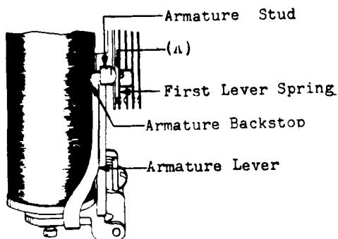
Fig. 17 - Illustrating Armature Stud Gap Requirement
