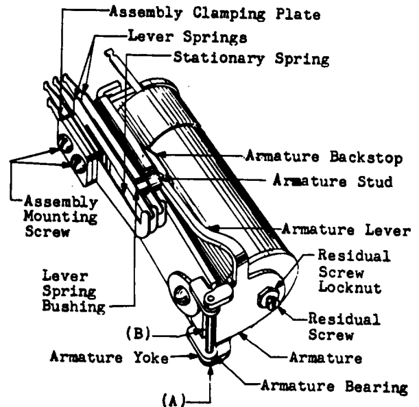
Fig. 6 - Pin-type Relay
