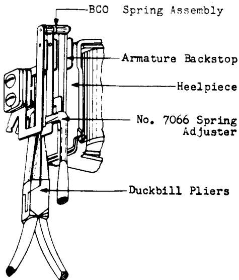
Fig. 31 - B Relay of Primary Line Switch - Method of Adjusting BCO Springs for Spring Gauging
