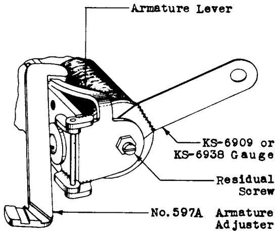
Fig. 25 - Method of Adjusting the Armature Lever
