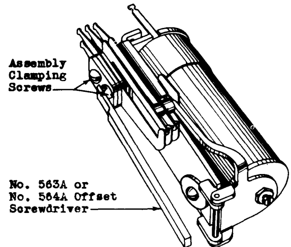
Fig. 21 - Aligning Contact Springs
