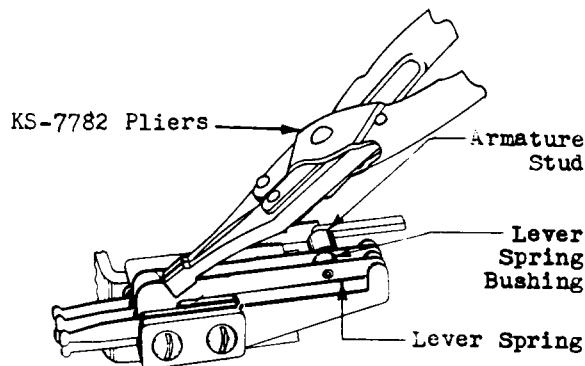
Fig. 30 - Removing Excessive Bow From Spring
