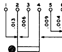
Fig. 20 - Typical Spring Combination to Which Exception 2.12(b)(4) Does Not Apply
