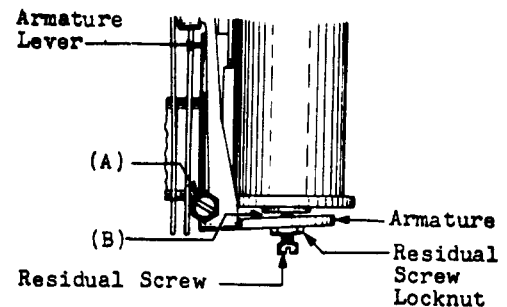
Fig. 7 - Pivot-type Relay
