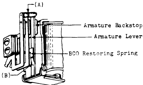
Fig. 18 - BCO Part of Primary Line Switch B Relay
