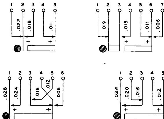
Fig. 19 - Typical Spring Combinations to Which Exception 2.12(b)(4) Applies
