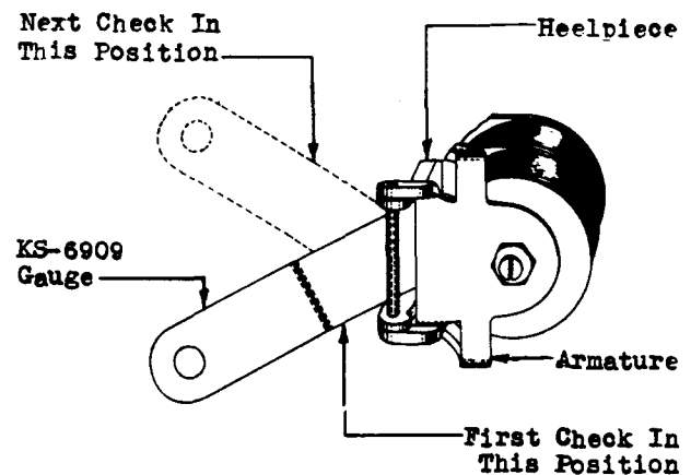
Fig. 9 - Checking Minimum and Maximum Heelpiece Airgap on Double Armature Relays and the Maximum Airgap on Single Armature Pin-type Relays
