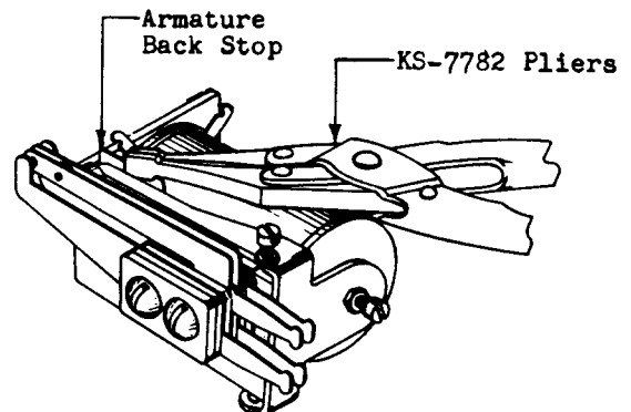
Fig. 27 - Adjusting the Armature Stud Gap on Relays Equipped With Pivot-type Armature
