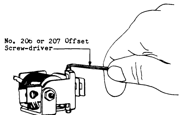
Fig. 22 - Method of Adjusting for Armature Movement
