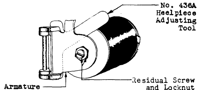
Fig. 23 - Adjusting the Heelpiece Airgap With the No. 436A Heelpiece Adjusting Tool Inserted From the Armature Side
