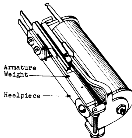
Fig. 3 - Pendulum-type Relay
