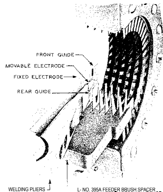
Fig. 4 - Welding Contact on Rear Feeder Brush Prong Using the No. 577A or 577B Welding Pliers
