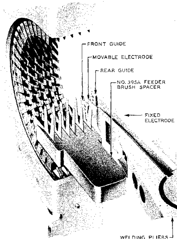
Fig. 5 - Welding Contact on Front Feeder Brush Prong Using No. 577A or 577B Welding Pliers
