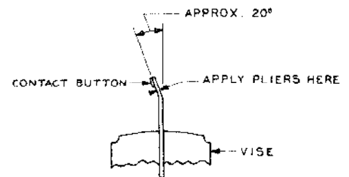
FIRST BEND
