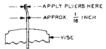
SECOND BEND
