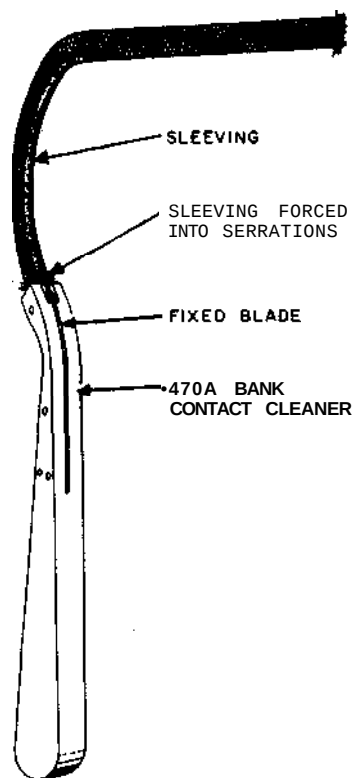
Fig. 2—New Sleeving Over Fixed Blade
