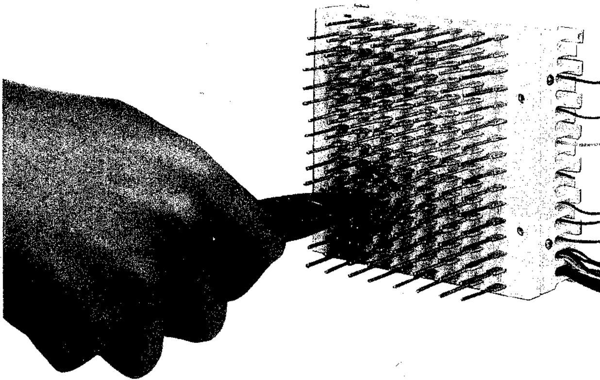
Fig. 2—Breaking Terminal From Block
