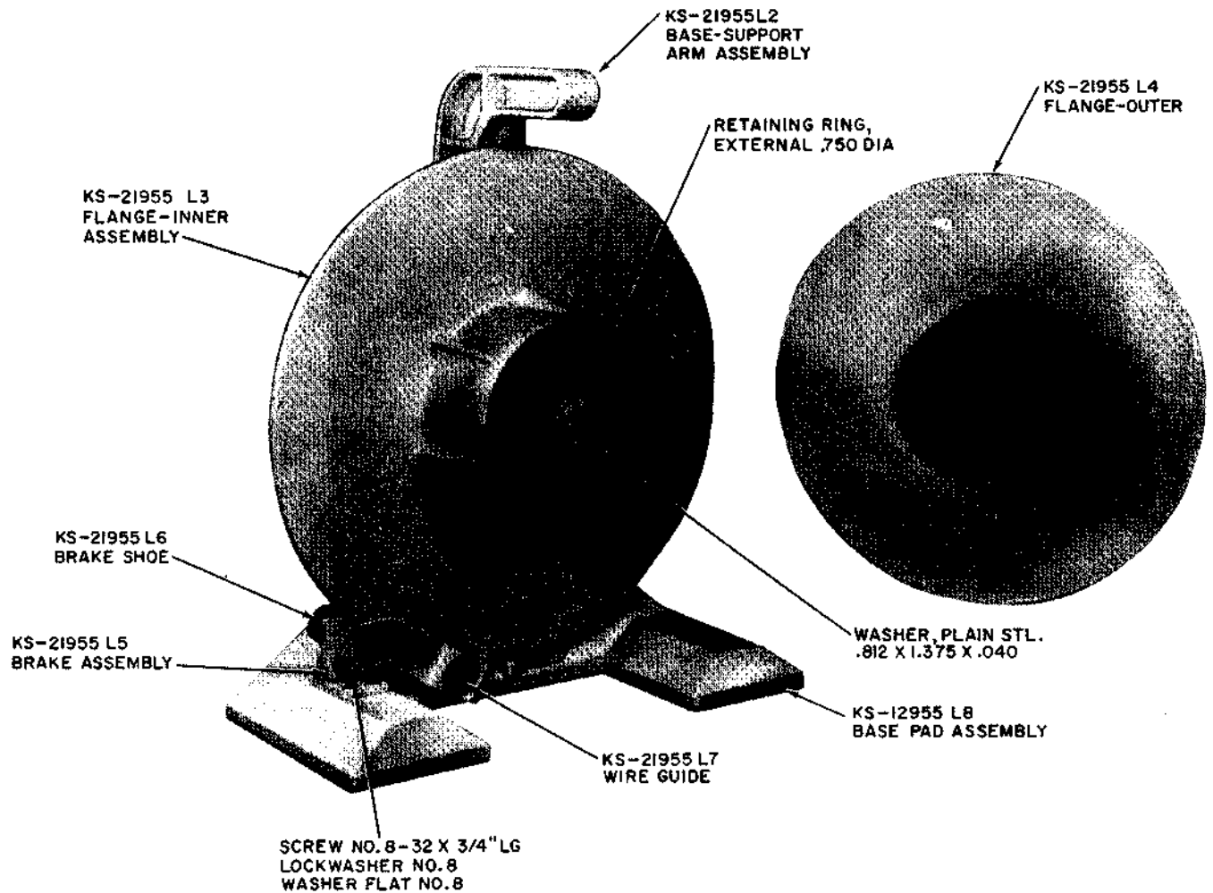
Fig. 2—KS-21955 Wire Reel With Outer Flange Removed
