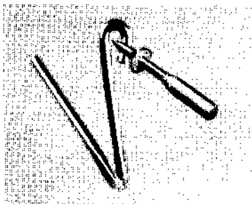
B Wire Loop with D Masonry Fastener
