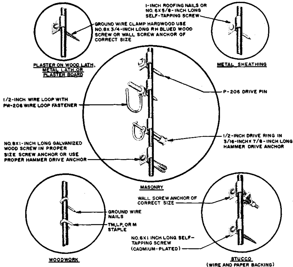
Fig. 17 – Fasteners for Ground Wire
