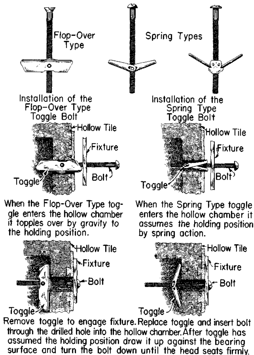
Fig. 32 — Toggle Bolts
