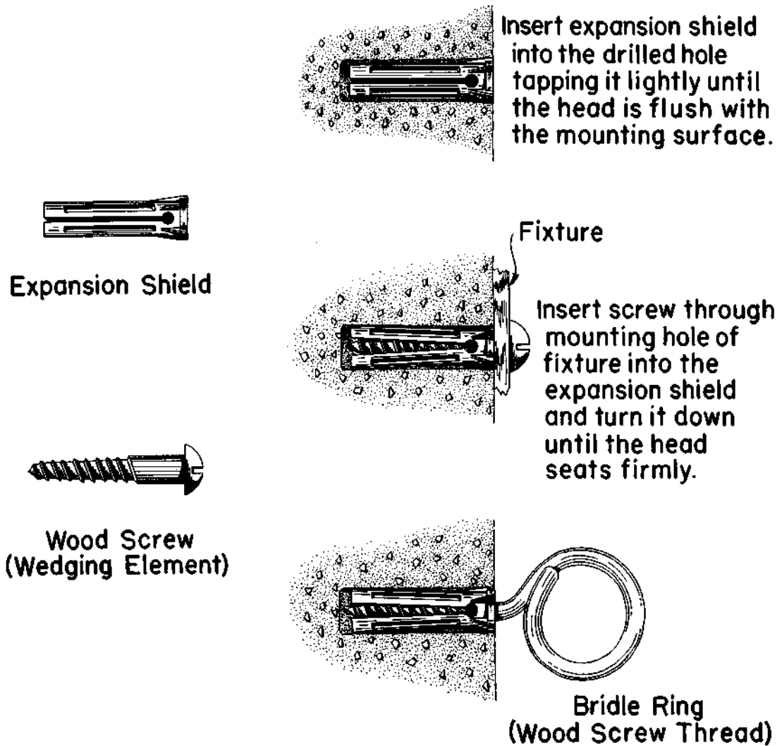
Fig. 20 — Wood Screw Anchors
