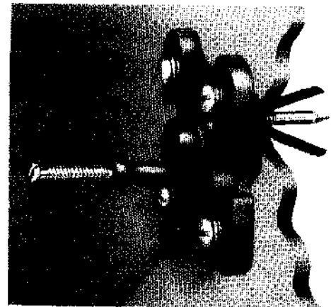
Fig. 28 — C Plastic Anchor, 42A Connecting Block
