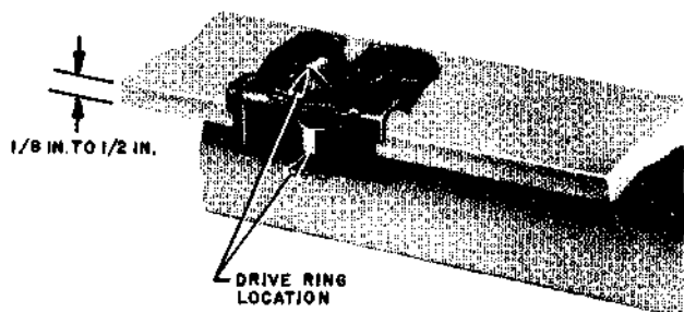
Fig. 10 — B Beam Clip, Bottom View
