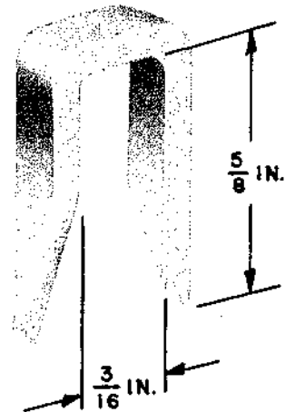
Fig. 2 – Ground Wire Staple
