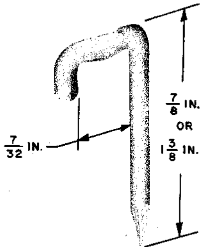
Fig. 1 – Ground Wire Nail
