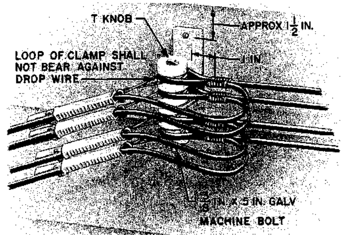
Fig. 3 — House Bracket Equipped with T Knob
