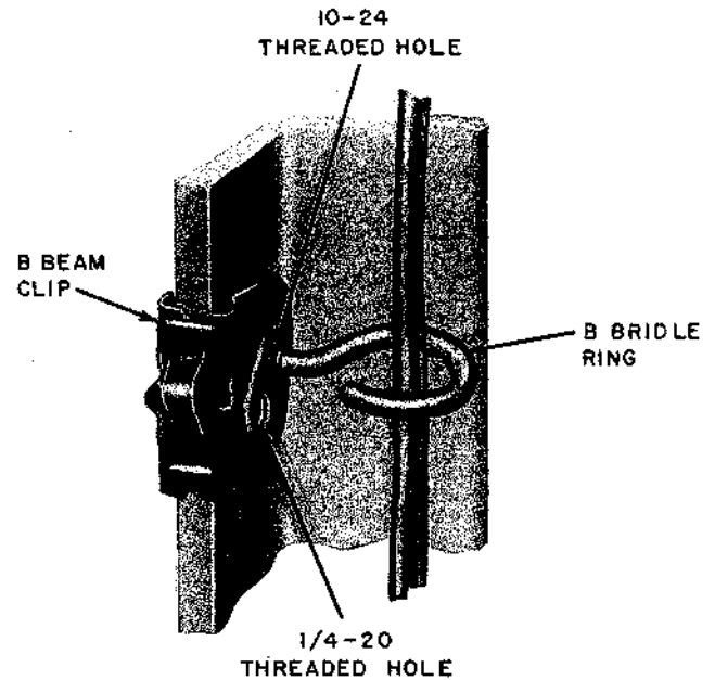
► Fig. 2—Installed K or M Bridle Ring Using B Insulator Support ◄
