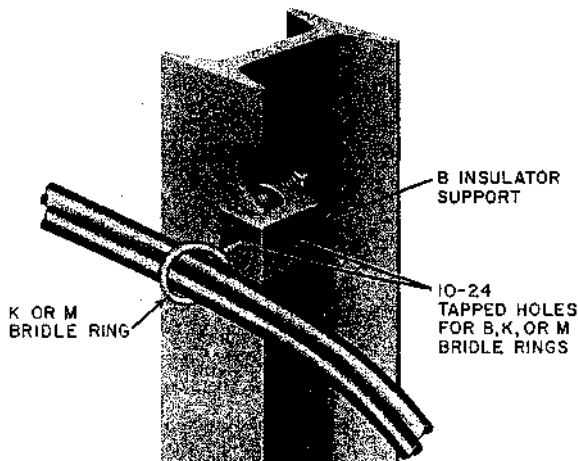
Fig. 1—Installed B Bridle Ring Using B Beam Clip
