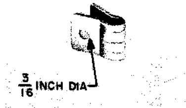
Fig. 1 - E Drop Wire Clamp
