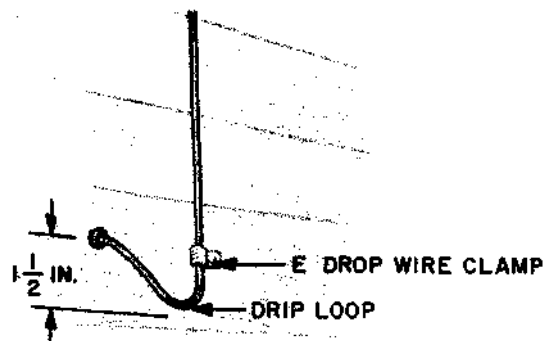
Fig. 2 - E Drop Wire Clamp Installed
