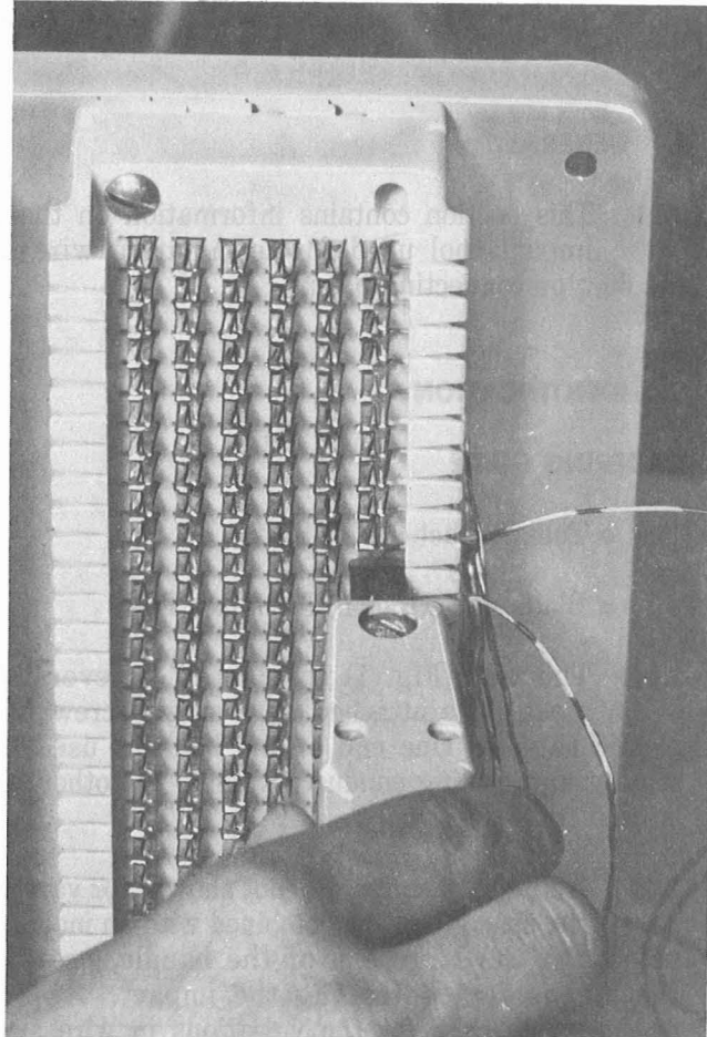
Fig. 2—Terminating or Looping Wire on 66-Type Connecting Block With B Impact Tool
