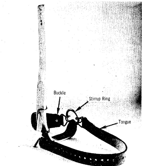
Fig. 5 – C Climber Foot Strap Installed on Right Climber
