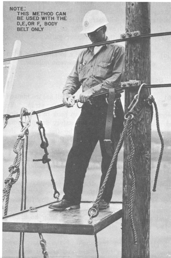
Fig. 9—Method of Using D, E, or F Body Belt With Safety Strap on Self-Supporting Cable
