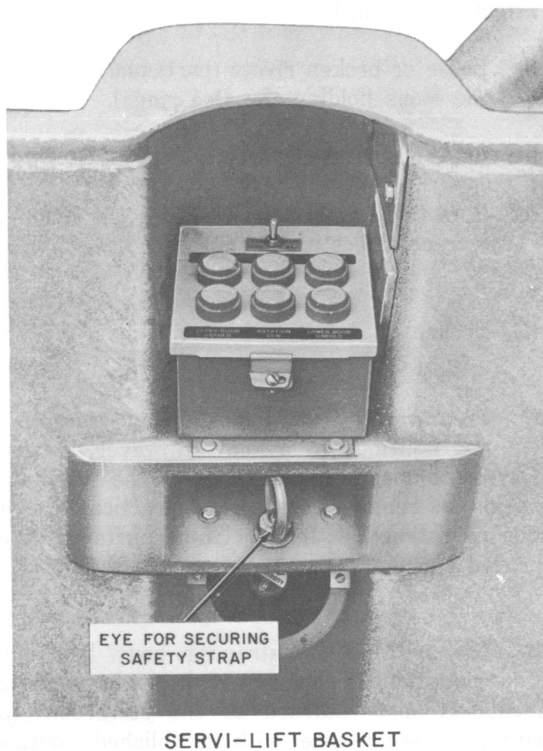
Fig. 10—Location of Eyes for Securing Safety Strap in Baskets of SKYWORKER and SERVI-LIFT Aerial Lifts
