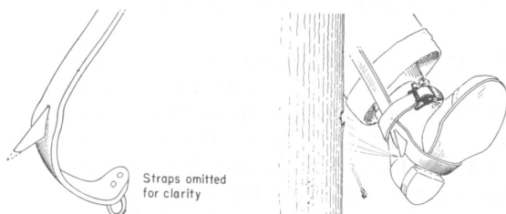
Fig. 12 — Dull Gaff
