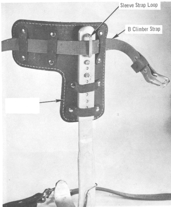
Fig. 6 — B Climber Pad (Right) Installed
