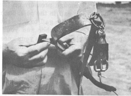
Fig. 18 — Removing Burrs from Top Cutting Edge
