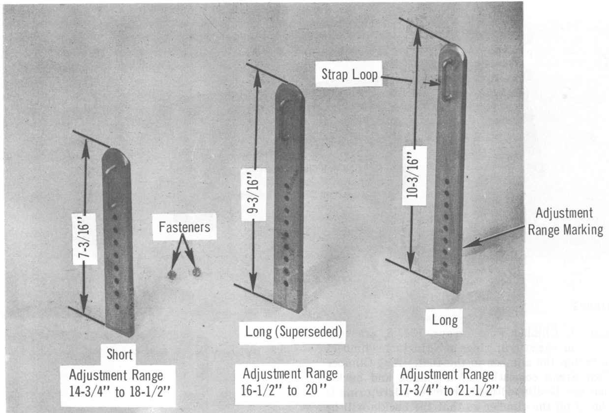
Fig. 3 — Sleeves for Adjustable Climbers
