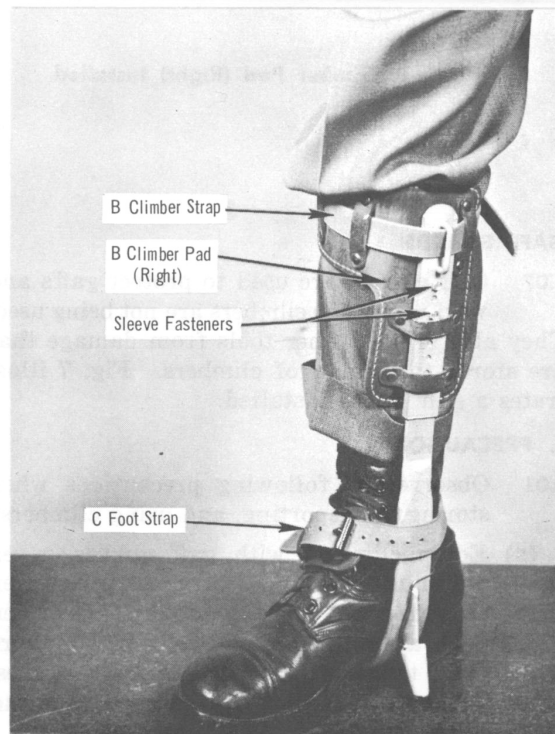
Fig. 9 — Right Climber on Leg
