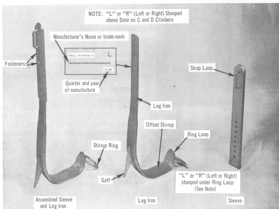
Fig. 1 — E Climber
