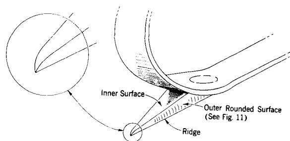
Fig. 10 — Gaff Profile and Point
