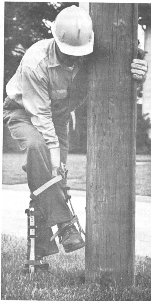
Fig. 14 — Jabbing Gaff in Pole
