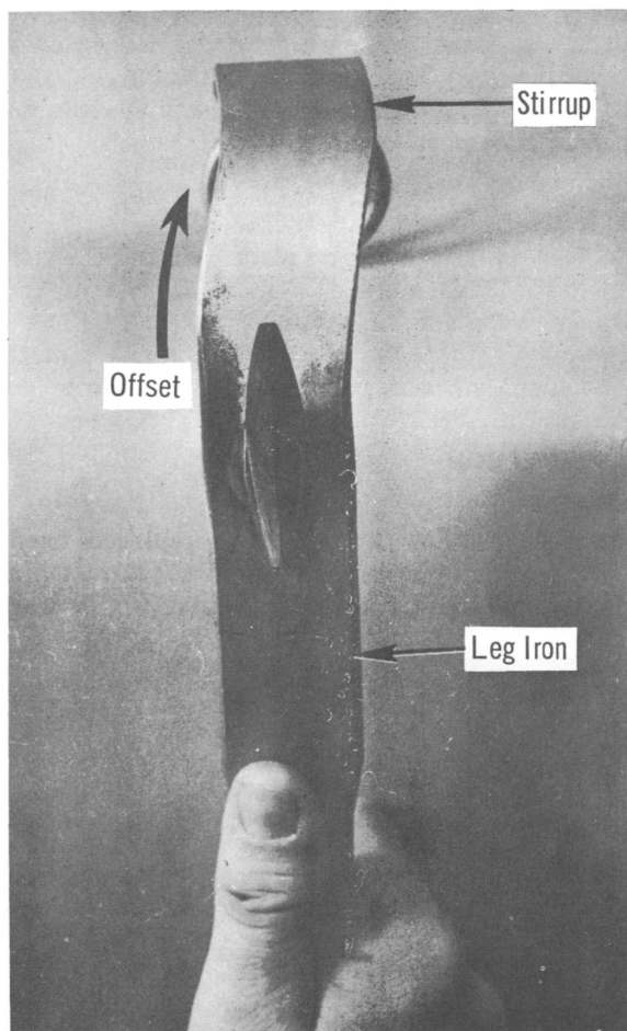
Fig. 2 — Stirrup Offset "Right"
