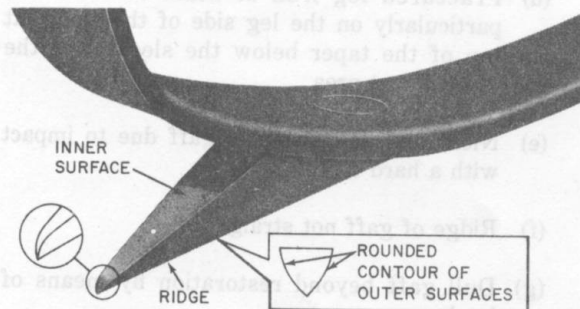
Fig. 10—Gaff Profile and Point
