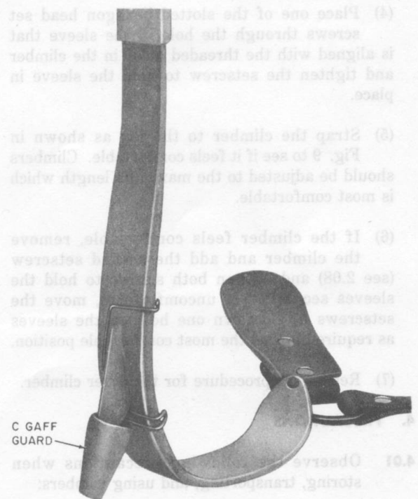
Fig. 7—C Gaff Guard Installed
