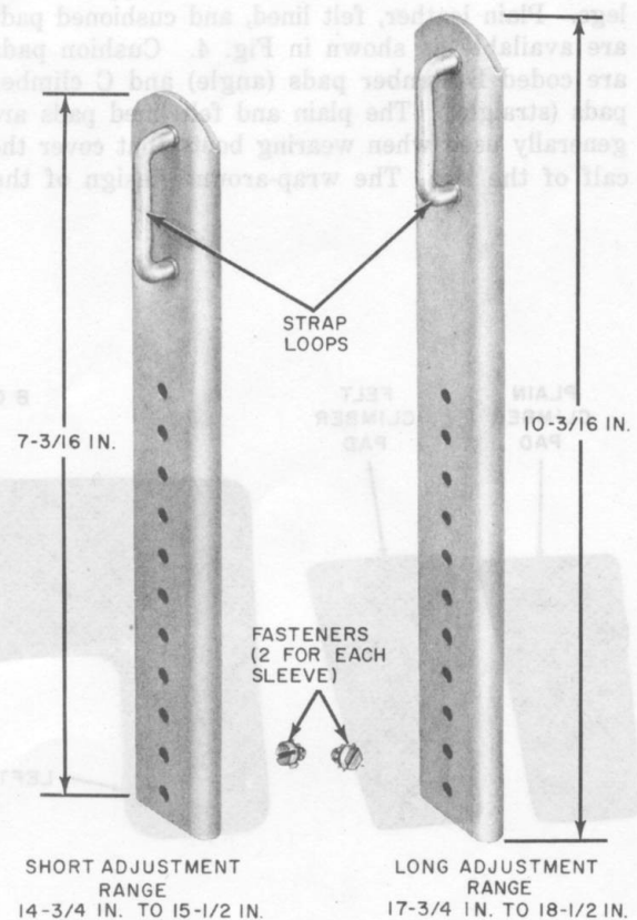
Fig. 3—Sleeves for Adjustable Climbers
