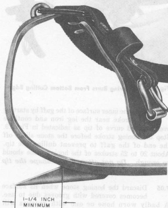
Fig. 21—Gaff Sharpened to Minimum Length
