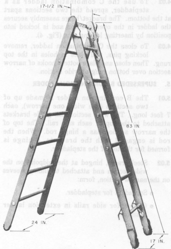
Fig. 1—C Combination Ladder (AT-8655)
