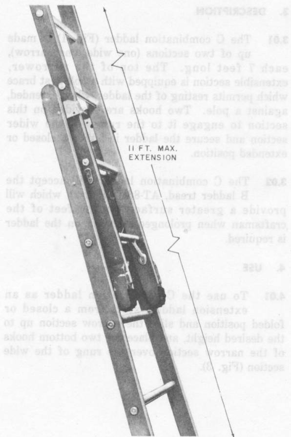
Fig. 3—C Combination Ladder in Extended Position
