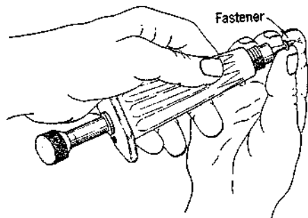
Fig. 5 – Fastener Placement
