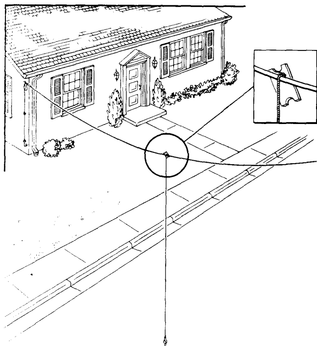
Fig. 15—Measuring Existing Drop With Clearance Measuring Line
