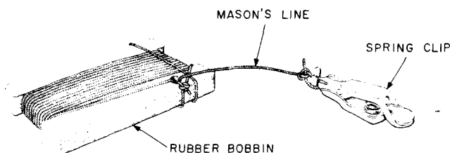
Fig. 12—Clearance Measuring Line
