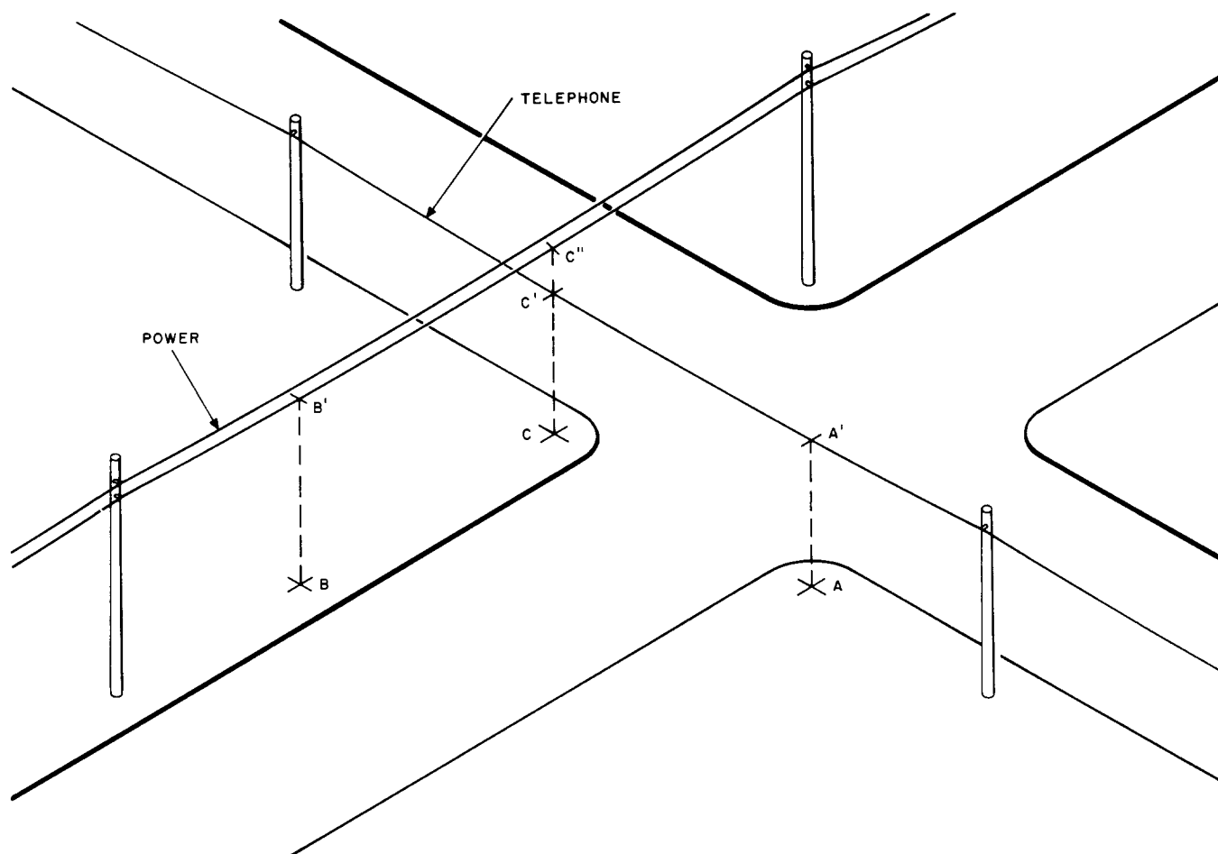
Fig. 4—Measuring Vertical Separation With Range Finder
