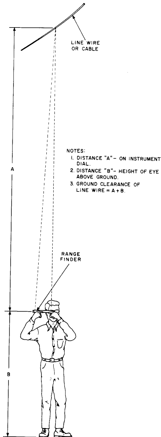
Fig. 3—Measuring Ground Clearance With Range Finder
