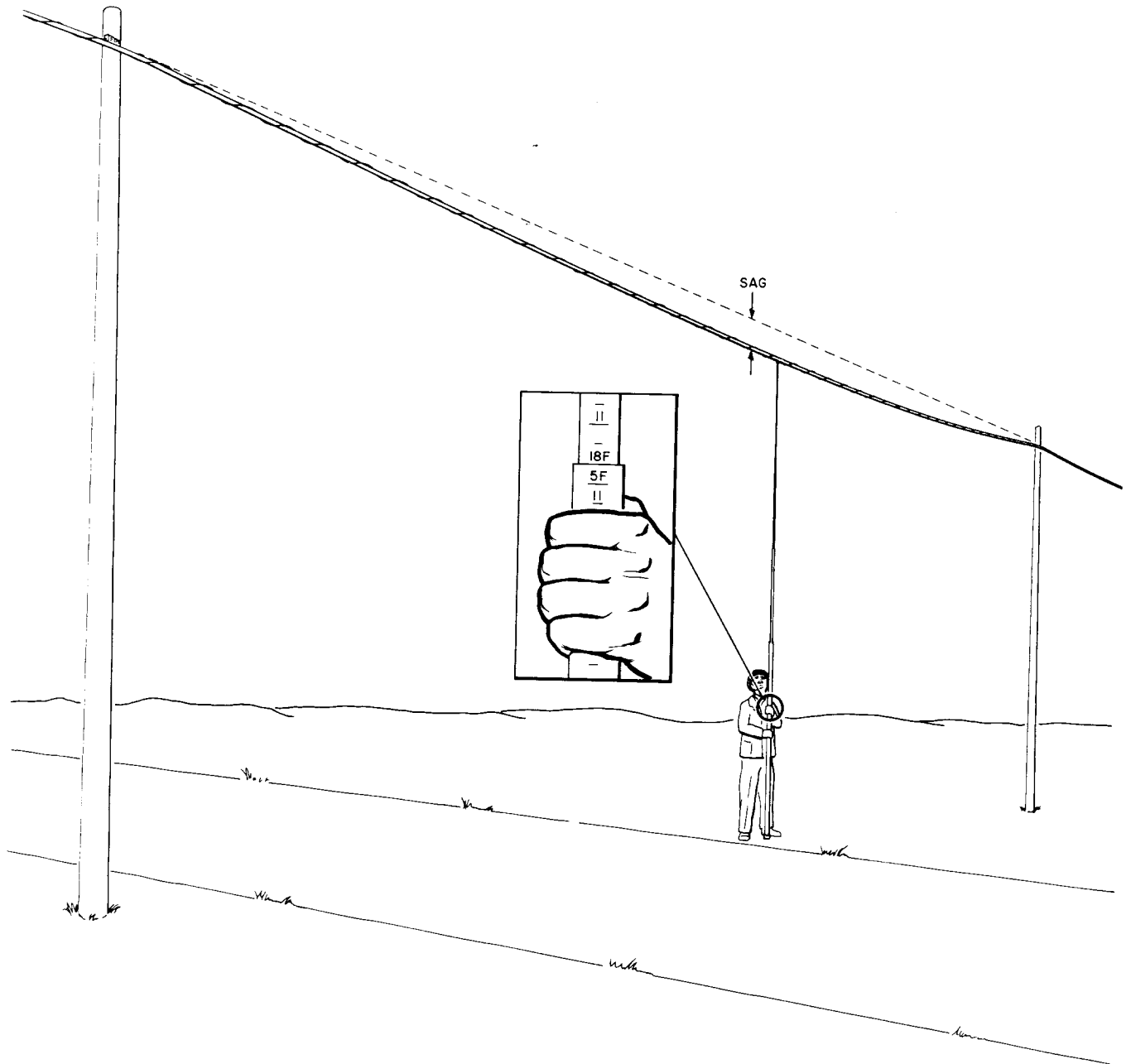
Fig. 18—Measuring Ground Clearance With B Clearance Rule
