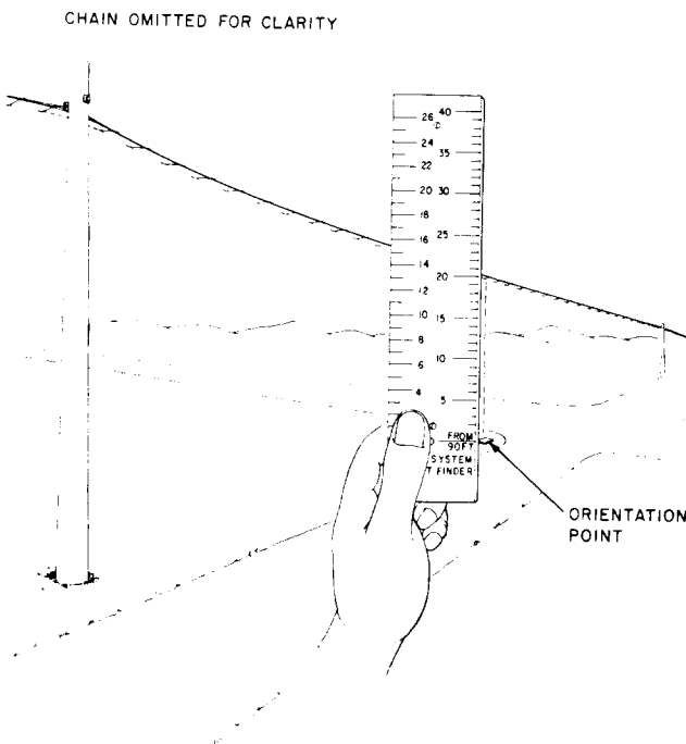
Fig. 10—Measuring Ground Clearance With B Height Finder
