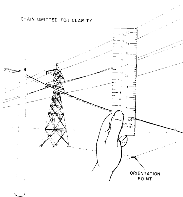
Fig. 9—Measuring Vertical Clearance With B Height Finder
