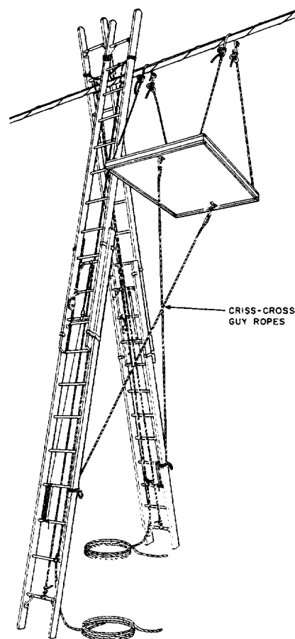
Fig. 17-Platform in Place and Lashed to Ladders
