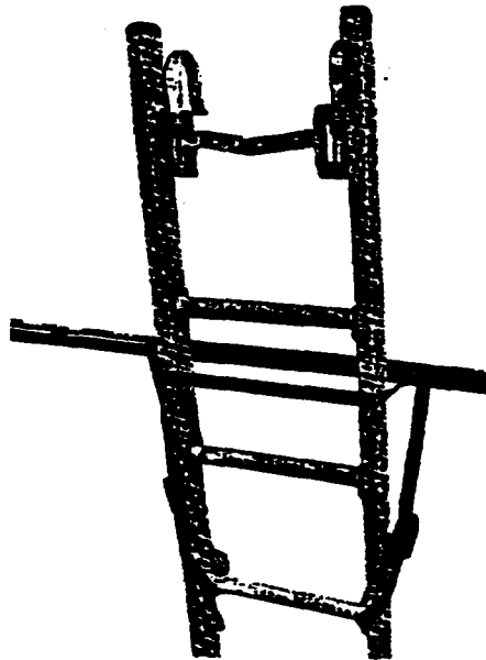
Fig. 8-Ladder Secured to Strand By Use of a Typical Top Ladder Lashing Device.
