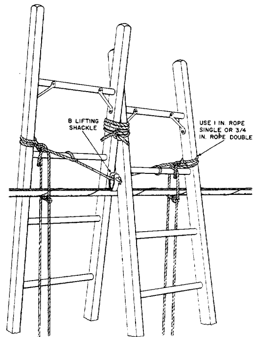
Fig. 17D-Rope Sling With B Lifting Shackle
