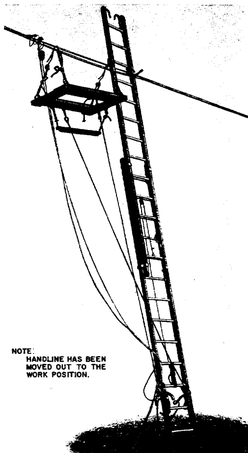
Fig. 16-D Platform Installed in Span
