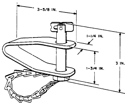
Fig. 17C-B Lifting Shackle
