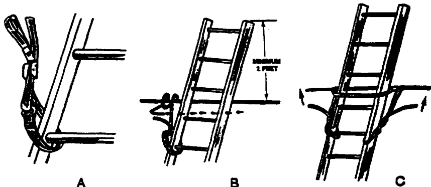
Figure 8-1. Securing Ladder to Strand, Using Top Ladder Lashing Device.
