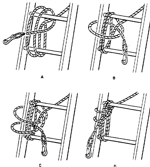
Fig. 15-Method of Tying Guy Ropes to Ladder
