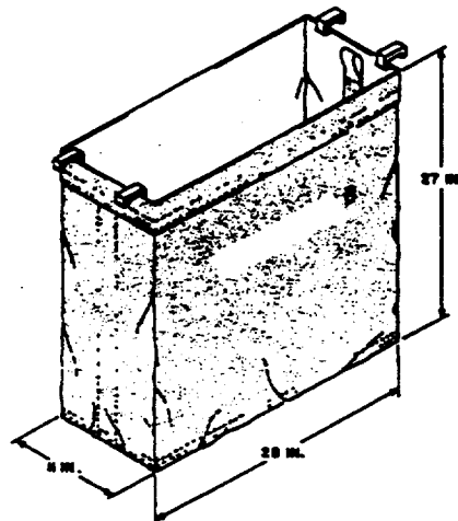
Fig. 2-B Platform Foot Bag
