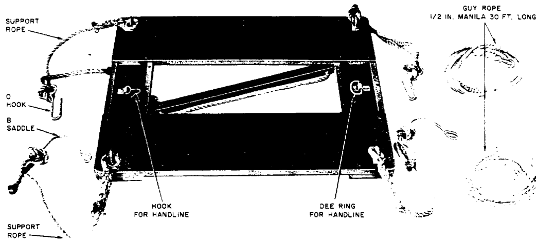
Fig. 1-D Aerial Platform
