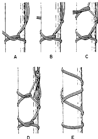
Fig. 14-Alternate Method of Tying Guy Ropes To Pole
