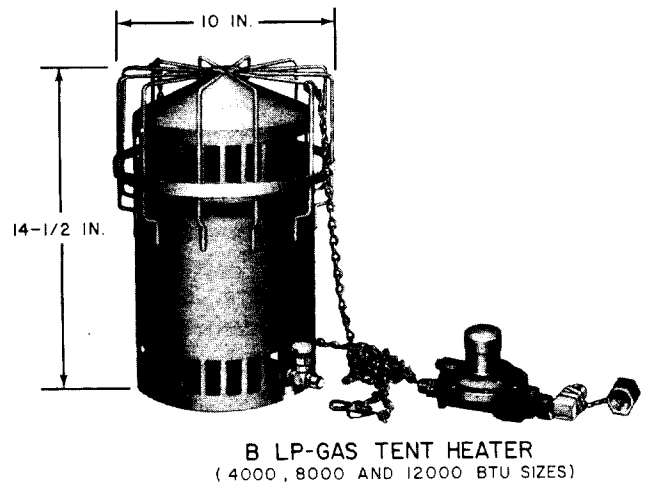
Fig. 1—B LP-Gas Tent Heater
