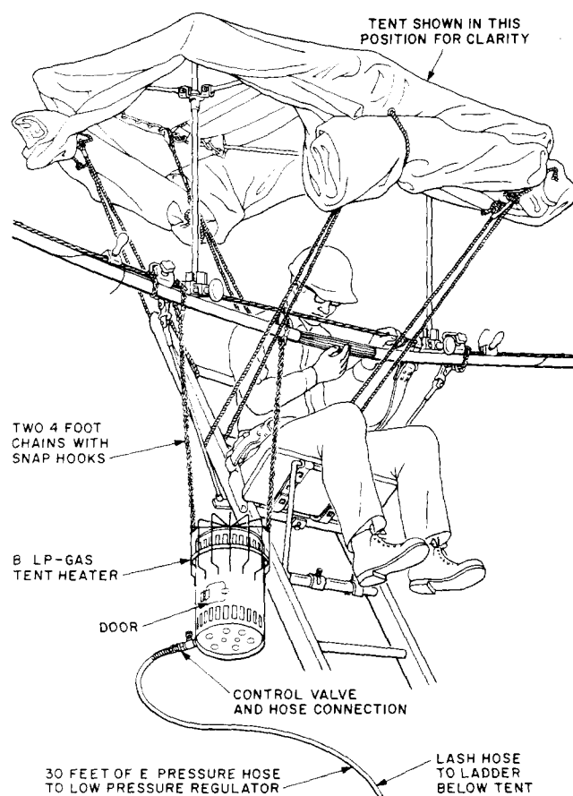
Fig. 3—Heater Attached to Strand
