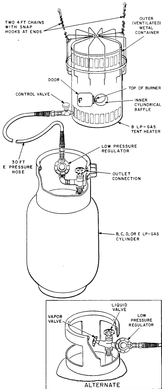
♦Fig. 2—Heater Connected to Cylinder♦
