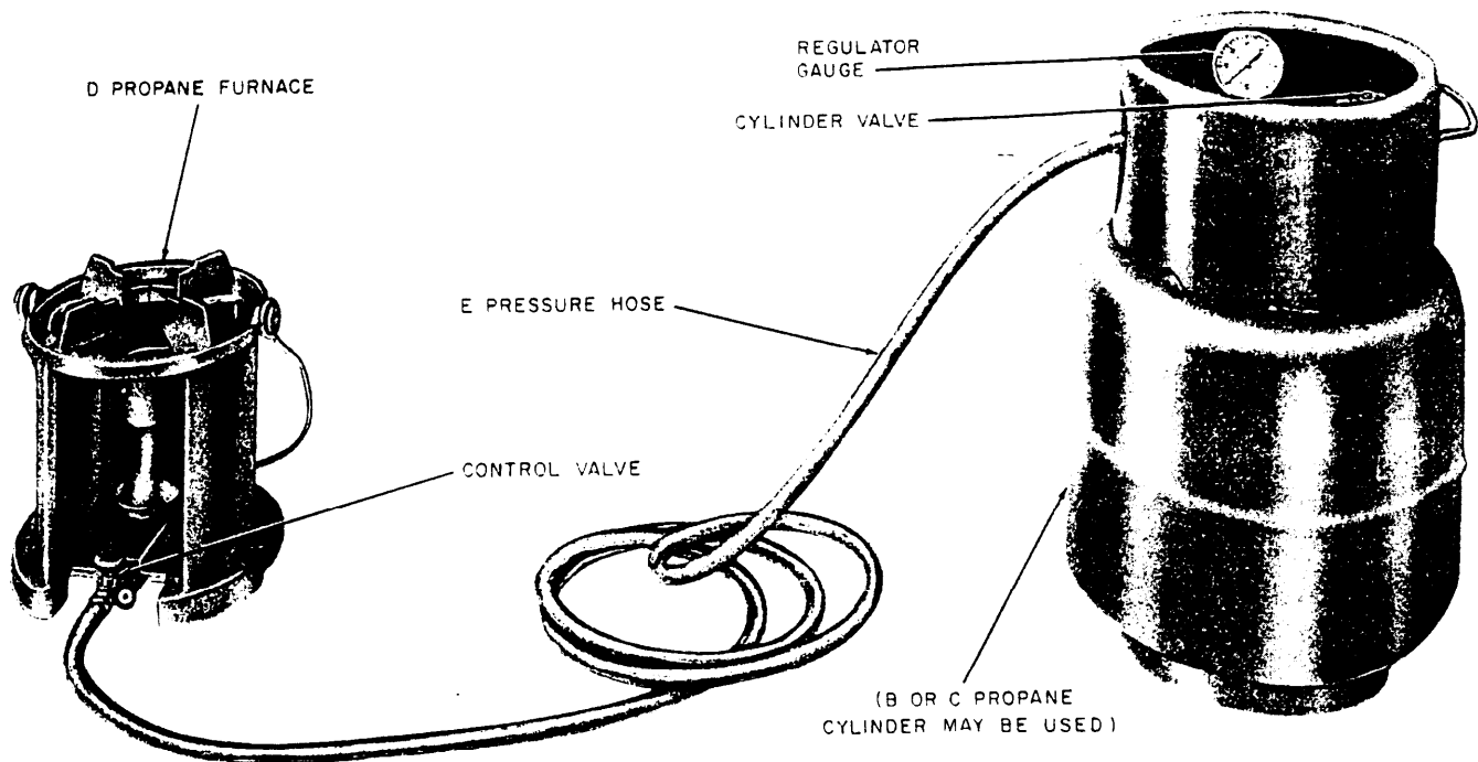
Fig. 4 - Typical Setup
